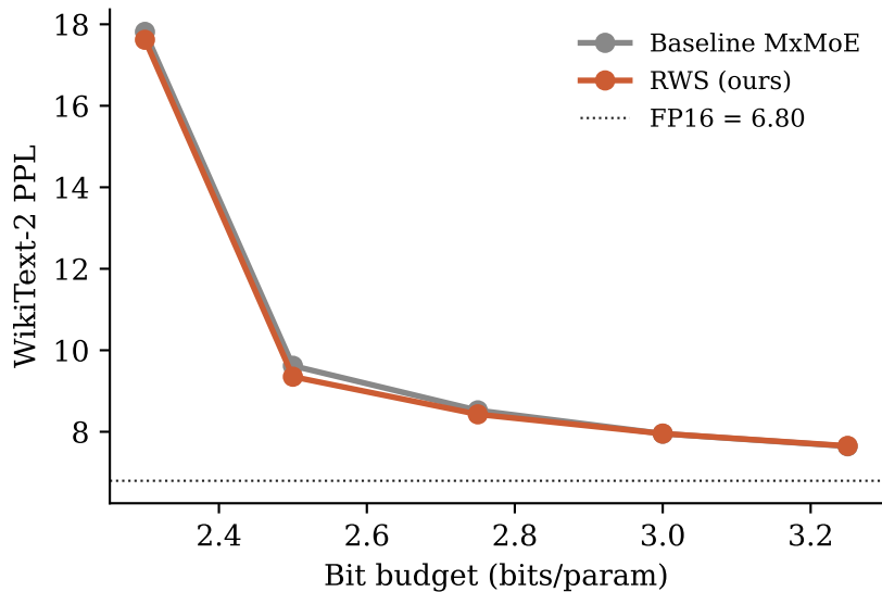
Qwen1.5-MoE-A2.7B (RHI=1.84)
