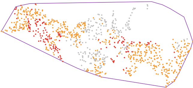
lambda6. Climate ~ Plant
