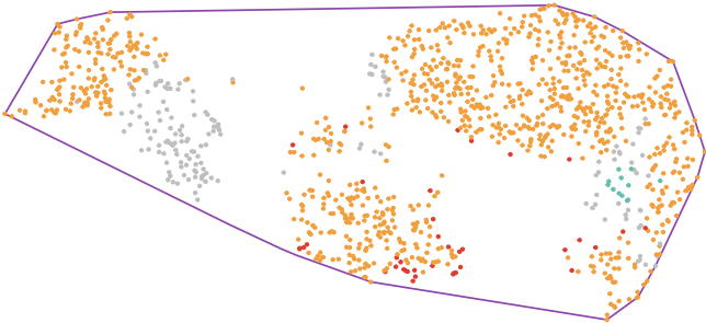
lambda4. NDVI == Plant
