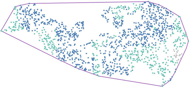
lambda5. Soil ~ Plant
