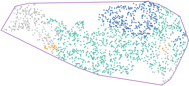
lambda3. Water content == Soil
