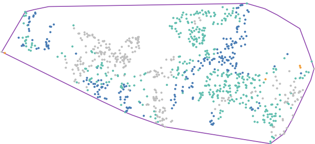
lambda7. Climate ~ Soil
