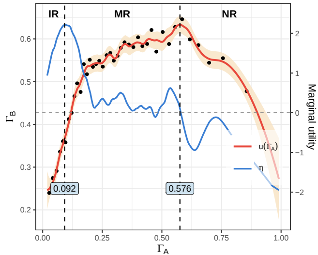
(b) Utility, marginal utility and DMU stages
