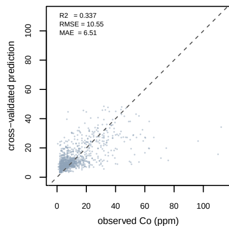
fold-level R2
