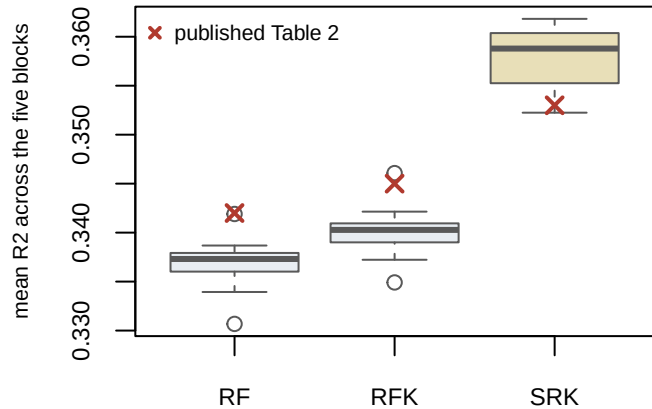
(a) Co: R2 over 20 forest seeds
