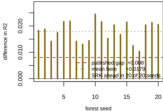
(b) Co: SRK minus RFK, seed by seed
