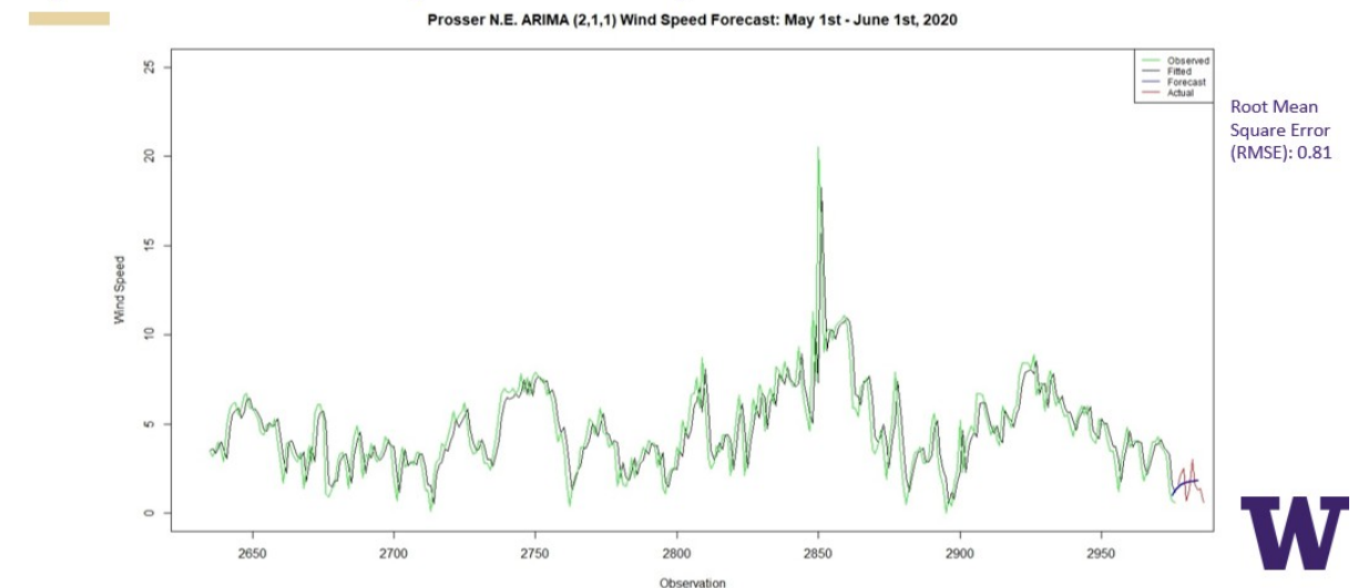
Figure 8: Short-term wind speed forecast using AgWeatherNet observations.
