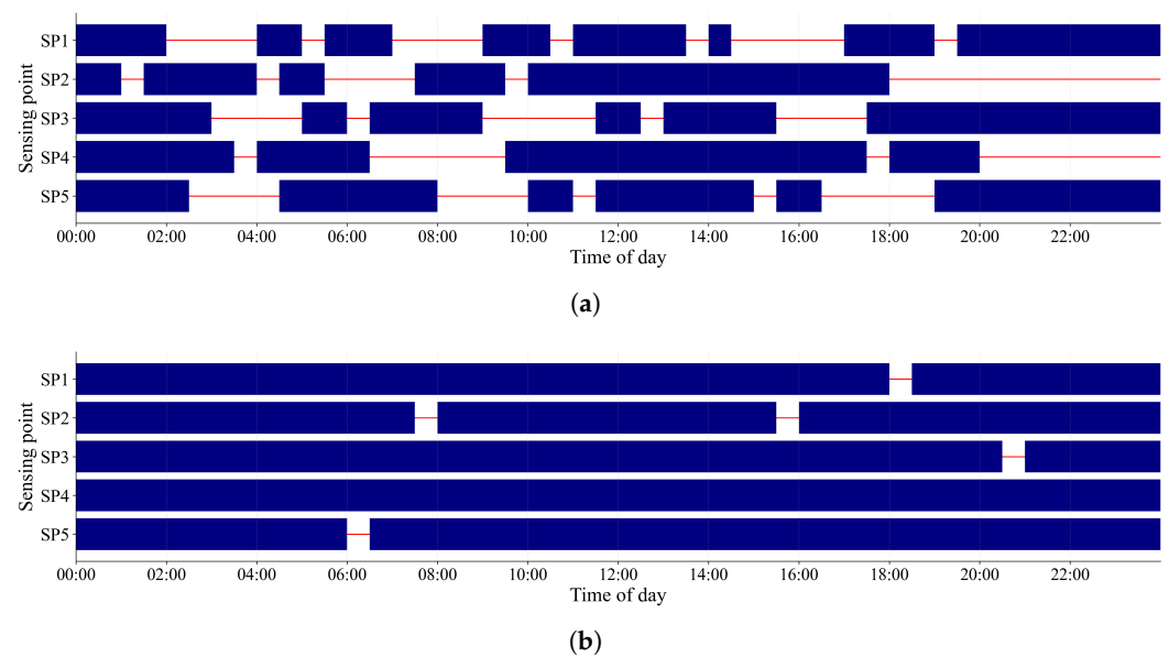
Figure 8. Reception stability across sensing points over time. (a) Before adjustment. (b) After adjustment.
