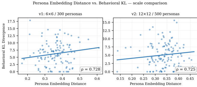
Fig. 5. Persona embedding distance vs. behavioral KL divergence at two scales (PCSP full). Left: v1 ( \rho = 0.728 ). Right: v2 ( \rho = 0.725 ). The monotone alignment between LLM semantic space and behavior space is preserved when moving to a 4\times larger grid with 4\times more agents and 67% more personas.
