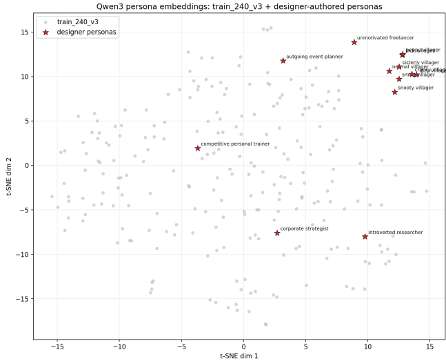
Fig. 3. Designer-authored personas in embedding space. A t-SNE projection of 240 training persona embeddings plus 13 designer-authored personas (stars) shows that the new personas lie within the region occupied by training personas rather than forming a separated out-of-distribution cluster. This supports the limited claim that the training data encompasses the tested designer-authored persona space.
