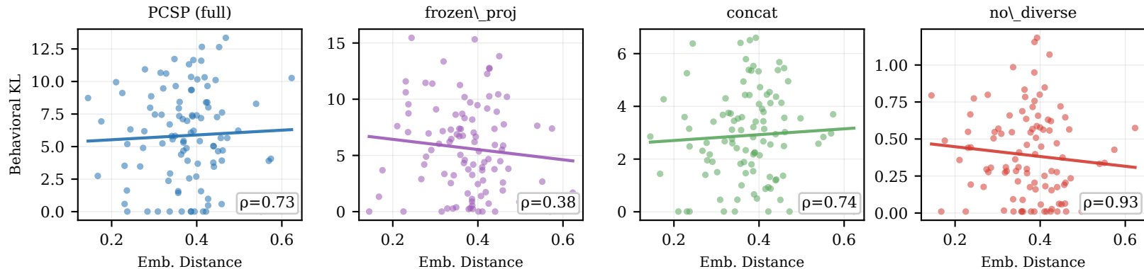
Fig 3 Persona Embedding Distance vs. Behavioral KL Divergence
