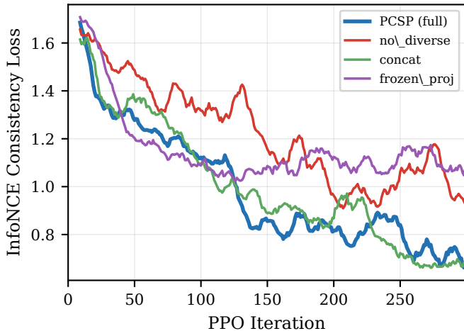
(b) Consistency Loss
