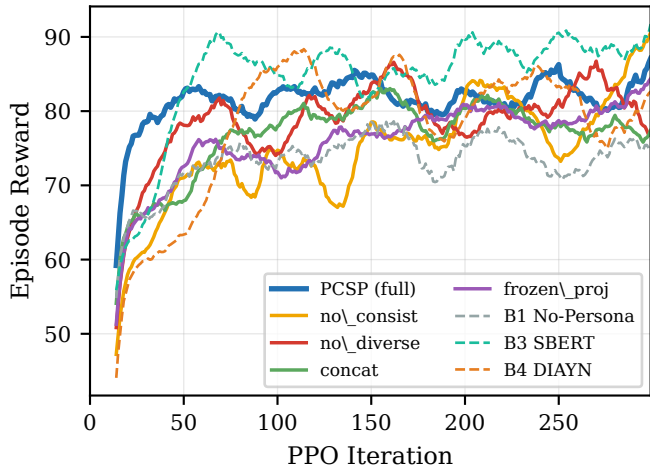
(a) Task Reward
