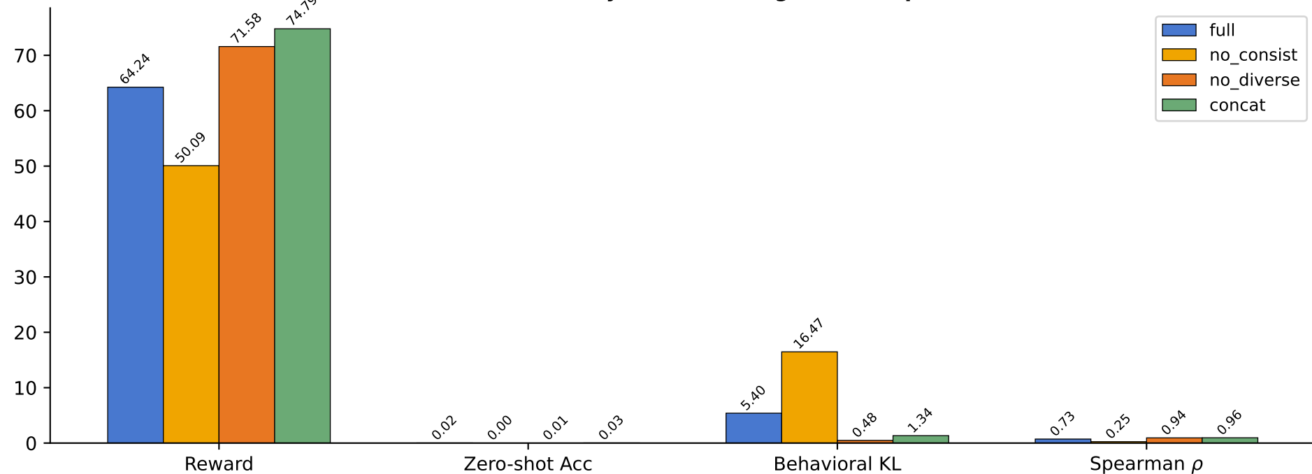
PCSP v2 Ablation Study (12×12, 16 agents, 500 personas)
