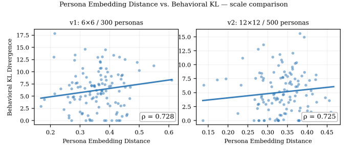
Fig. 5. Persona embedding distance vs. behavioral KL divergence at two scales (PCSP full). Left: v1 ( \rho = 0.728 ). Right: v2 ( \rho = 0.725 ). The monotone alignment between LLM semantic space and behavior space is preserved when moving to a 4\times larger grid with 4\times more agents and 67% more personas.
