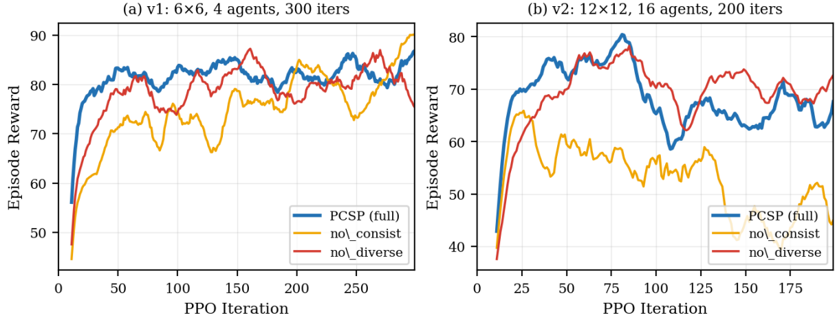
Fig. 10. Training reward curves at two scales. (a) v1 (6×6, 4 agents, 300 iters). (b) v2 (12×12, 16 agents, 200 iters). Removing the consistency loss (no_consist) preserves or even slightly increases reward but collapses zero-shot persona traceability across all scales (Tables XI–III). Removing the diversity loss (no_diverse) causes KL collapse at v1 and v2 (0.39 and 0.48) and a v1 reward drop, but its effect on v3 zero-shot accuracy is within the Wilson CI of full (§V).
