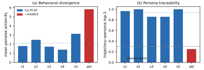
Fig. 4. Melting Pot single-substrate detail on commons_harvest__open . Per-seed bars (blue: full pcp, 5 seeds; red: -InfoNCE ablation, 1 seed). Dotted blue line: 5-seed mean. (a) Mean pairwise action-KL across the \binom{10}{2} = 45 persona pairs. (b) In-distribution trajectory \rightarrow persona top-3 retrieval on the 10-train vocabulary (dashed grey: chance 3/10 ). The ablation reaches the highest KL but the lowest top-3 (below chance): policies are different yet trajectories no longer encode which persona produced them. The two additional substrates in Tab. VI replicate this pattern.
