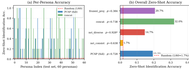
Fig. 14. Zero-shot generalization on 60 unseen personas (v1). PCSP (full) achieves 19.3% trajectory-to-persona identification; the red dashed line marks random chance (1.7%). Removing the consistency loss collapses accuracy to 1.7%. The v2 experiment (100 unseen personas) replicates this qualitative pattern.
