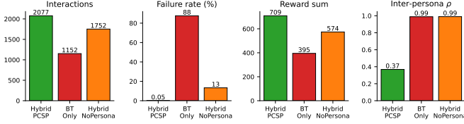
Fig. 8. Phase 4 runtime ablation, 64 agents. Zeroing the persona embedding (HybridNoPersona) collapses inter-persona action dispersion from \rho = 0.37 to \rho = 0.99 . Replacing the ONNX policy with the BT-only needs heuristic (BTOnly) further halves throughput and reward as 64 agents synchronise on the single most-urgent need each tick.
