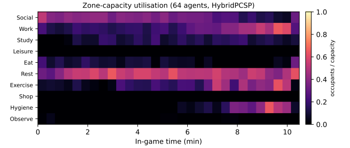
Fig. 10. Zone-capacity utilisation over a 64-agent HybridPCSP episode. Per-zone occupants/capacity (rows) across 30 equal time bins over the \sim 10.5 -min episode (columns). Rest, Work, Hygiene, and Exercise zones carry the load (peaks \approx 0.65 ); the unevenness is the engine-side contention behind the \rho -drop.
