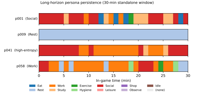
Fig. 9. Long-horizon persona persistence (Layer 3). Per-minute dominant intent category for four maximally-separated personas over 30 in-game minutes in UE5 (8 agents, frozen Layer-1 checkpoint, 0.5s decision throttle, 0.0% BT-abort). Each row is one persona; each column is a 1-minute bin coloured by the modal intent category. p009 stays in Rest for all 30 bins (single run); p058 holds Work as its modal axis in 17/30 bins; p001 is Social-dominant (15/30 bins) while cycling through five categories; p041 splits evenly between Social and Work. No persona ever “forgets” its dominant axis over the 30-minute window.
