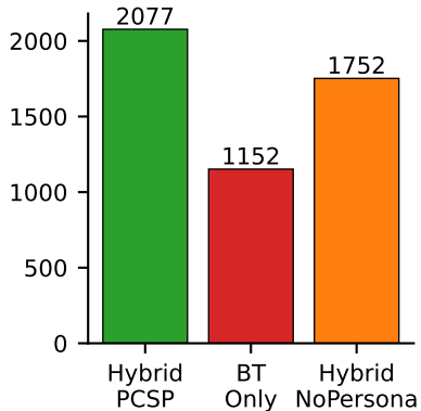
Interactions
