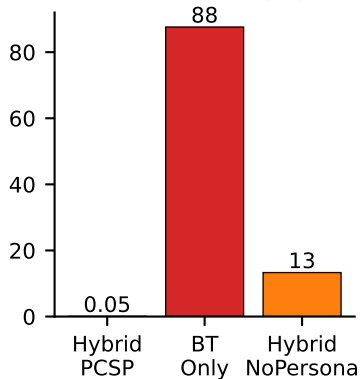
Failure rate (%)
