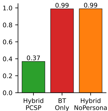
Inter-persona \rho
