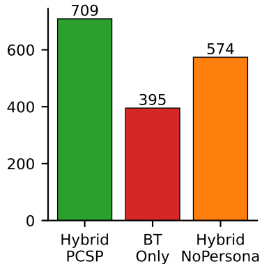
Reward sum
