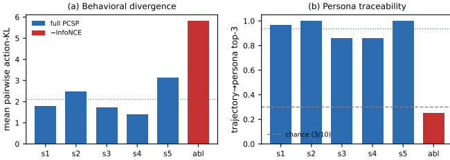
Fig. 6. Melting Pot external check on commons_harvest__open . Per-seed bars (blue: full PCSP, 5 seeds; red: –InfoNCE ablation, 1 seed). Dotted blue line: 5-seed mean. (a) Mean pairwise action-KL across the \binom{10}{2}=45 persona pairs. (b) In-distribution trajectory→persona top-3 retrieval on the 10-train vocabulary (dashed grey: chance 3/10). The ablation reaches the highest KL but the lowest top-3 (below chance): policies are different yet trajectories no longer encode which persona produced them.
