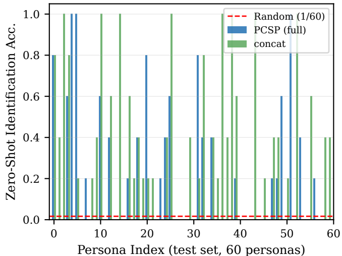
(a) Per-Persona Accuracy
