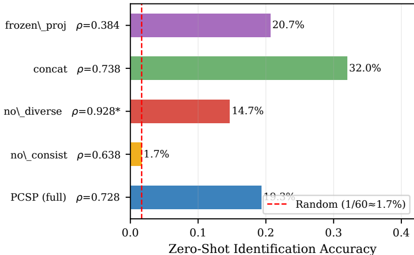
(b) Overall Zero-Shot Accuracy
