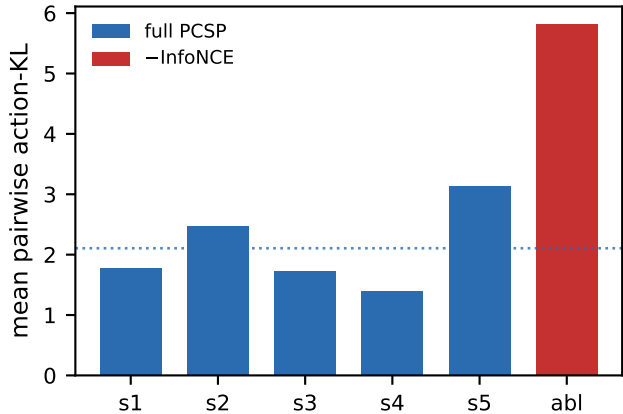
(a) Behavioral divergence
