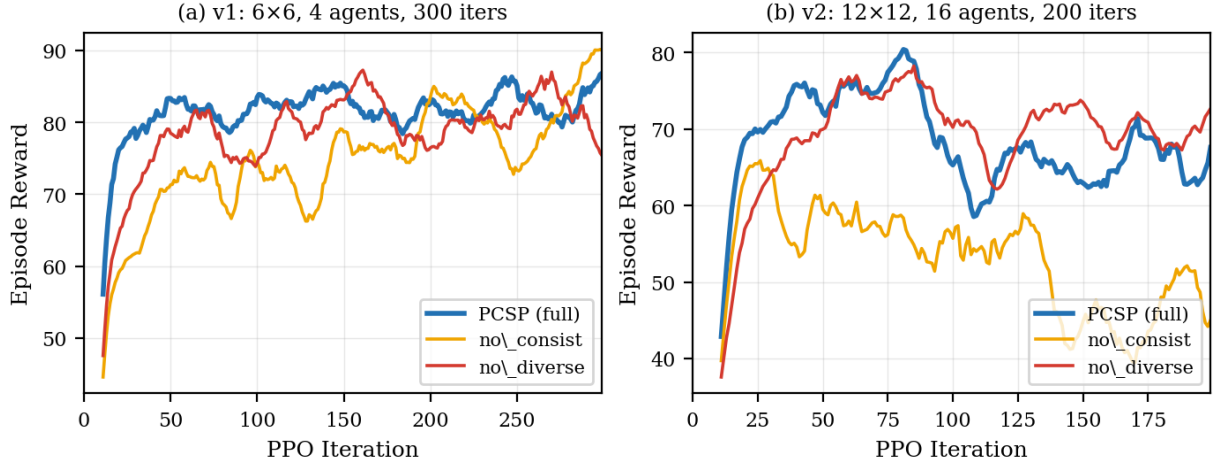
Fig. 13. Training reward curves at two scales. (a) v1 (6×6, 4 agents, 300 iters). (b) v2 (12×12, 16 agents, 200 iters). Removing the consistency loss (no_consist) preserves or even slightly increases reward but collapses zero-shot persona traceability across all scales (Tables XII–III). Removing the diversity loss (no_diverse) causes KL collapse at v1 and v2 (0.39 and 0.48) and a v1 reward drop, but its effect on v3 zero-shot accuracy is within the Wilson CI of full (§V).
