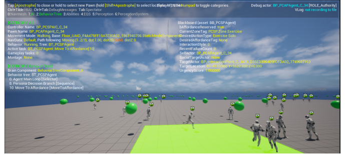
Fig. 7. Gameplay Debugger overlay on a single agent. Yellow text (right) is the live Blackboard / BT snapshot for the selected APCSPAgentCharacter: current DesiredActionType, UrgencyScore, bAffordanceReserved, and the active BT node. This view confirms that the persona branch is routing decisions through BTTask_PCSPDecision → MoveToAffordance → PerformInteraction and that the emergency decorator fires only when UrgencyScore ≥ 0.85.
