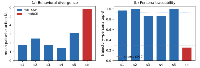
Fig. 4. Melting Pot single-substrate detail on commons_harvest__open. Per-seed bars (blue: full PCSP, 5 seeds; red: -InfoNCE ablation, 1 seed). Dotted blue line: 5-seed mean. (a) Mean pairwise action-KL across the \binom{10}{2}=45 persona pairs. (b) In-distribution trajectory \rightarrow persona top-3 retrieval on the 10-train vocabulary (dashed grey: chance 3/10 ). The ablation reaches the highest KL but the lowest top-3 (below chance): policies are different yet trajectories no longer encode which persona produced them. The two additional substrates in Tab. VI replicate this pattern.
