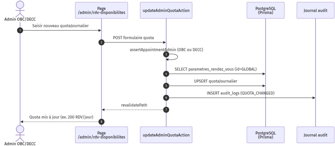
Figure 3.31 — Séquence quota RDV
