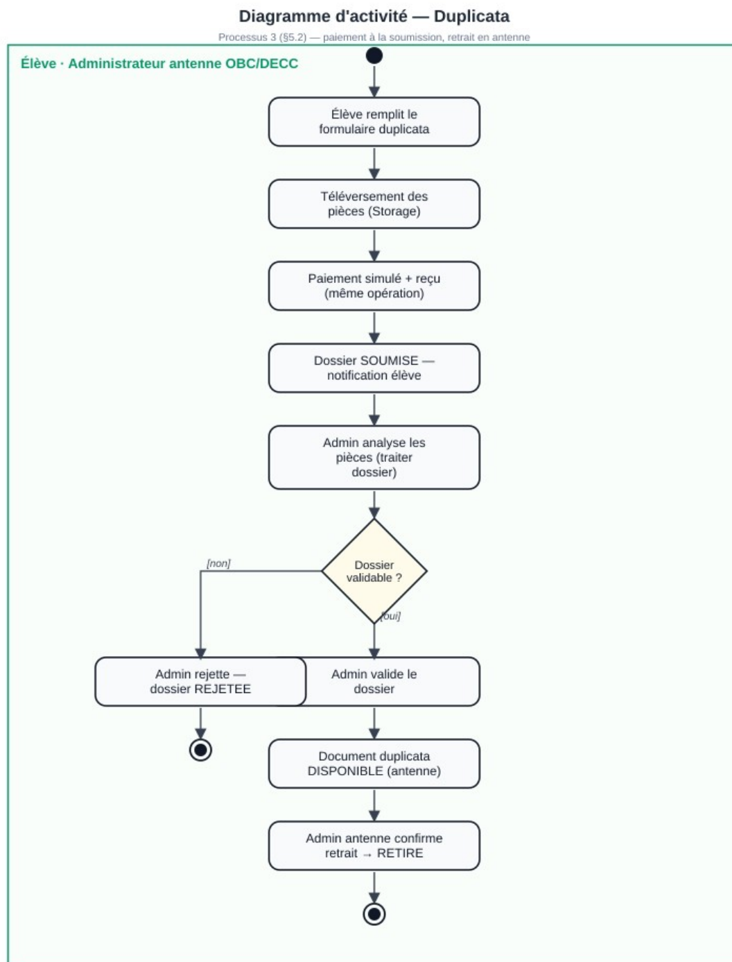
Figure 3.39 — ACT-02 duplicata
