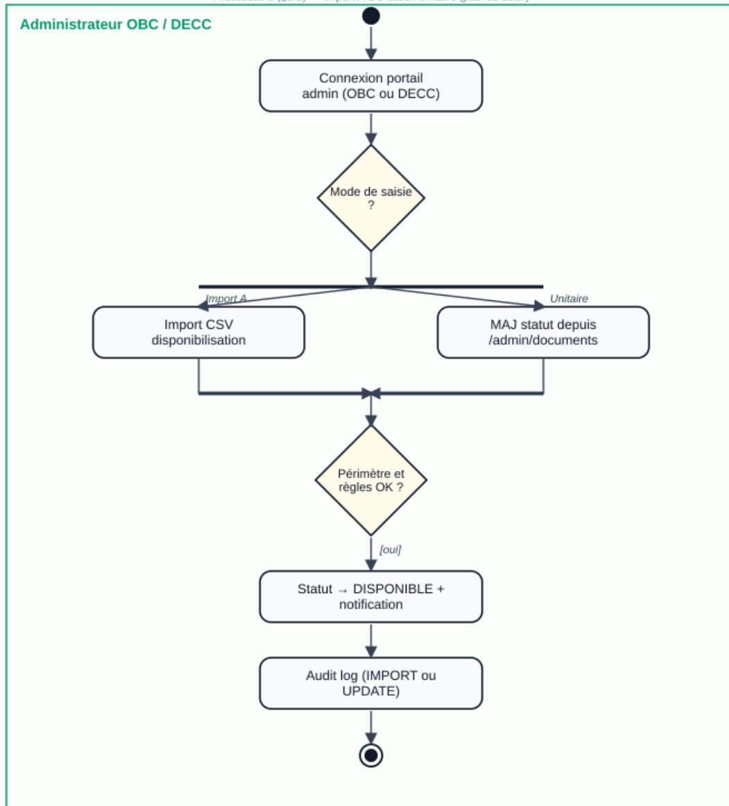
Figure 3.40 — ACT-03 disponibilisation
