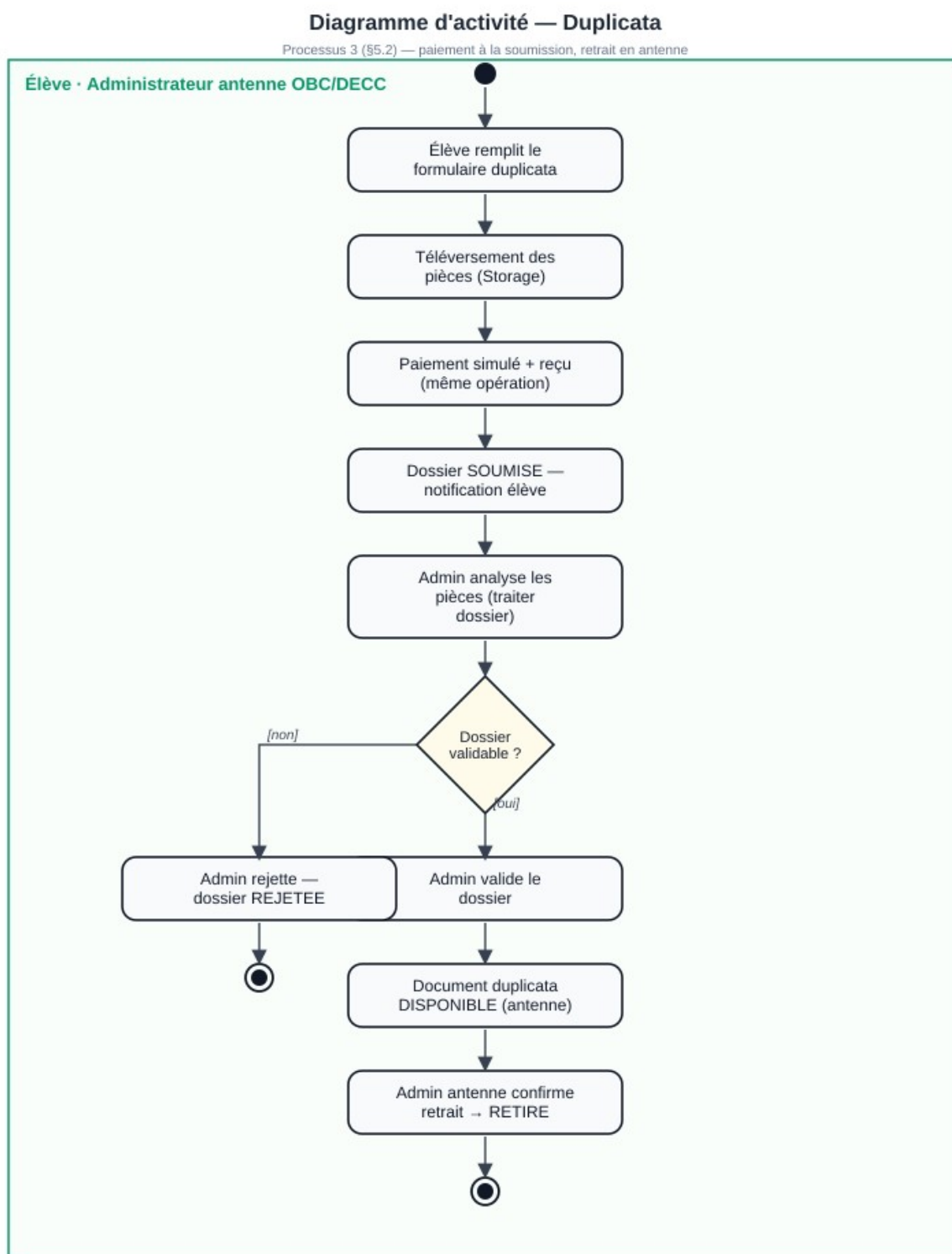
Figure 3.39 — ACT-02 : processus duplicata
