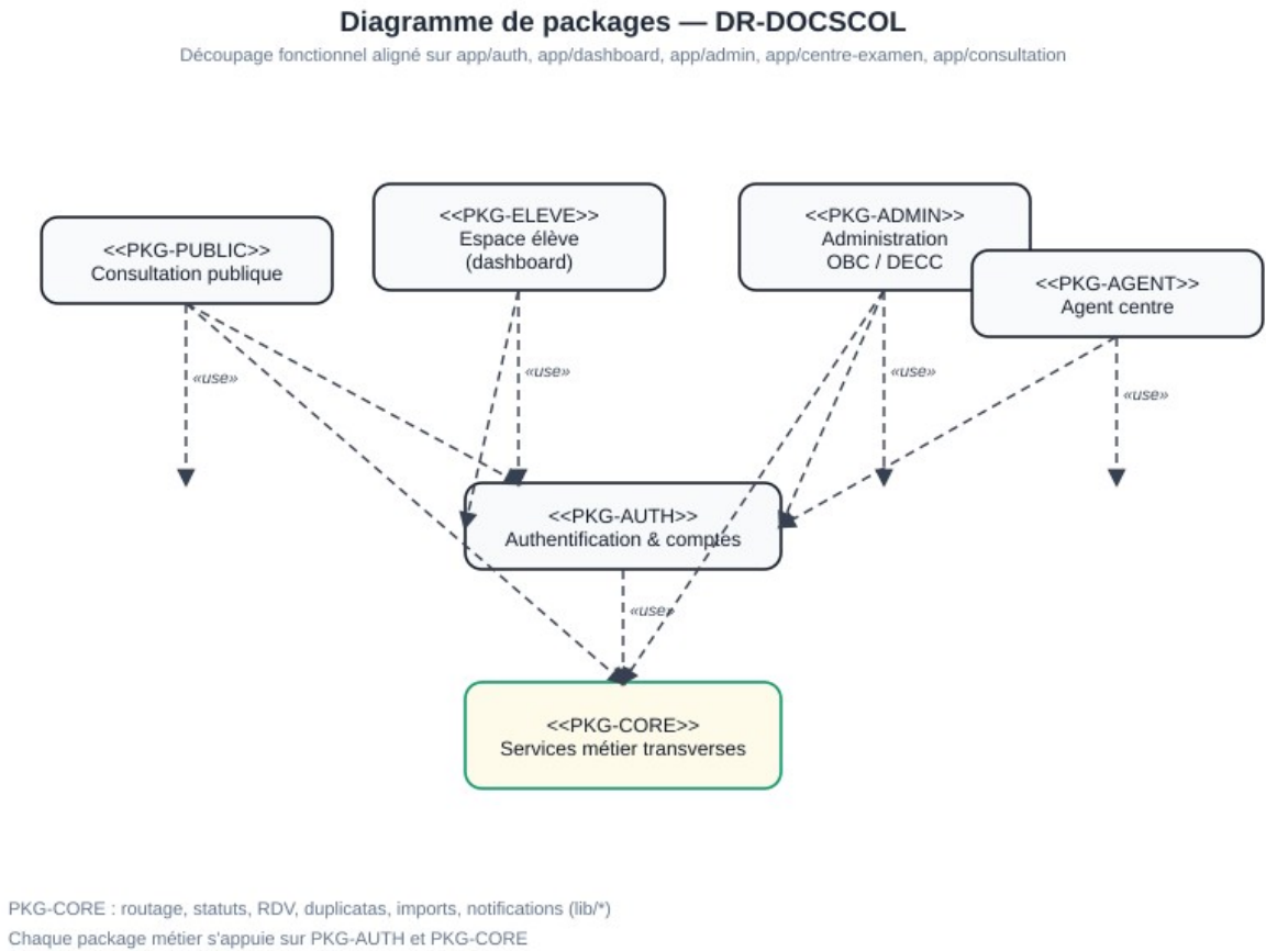
Figure 2.3 — Diagramme de packages
