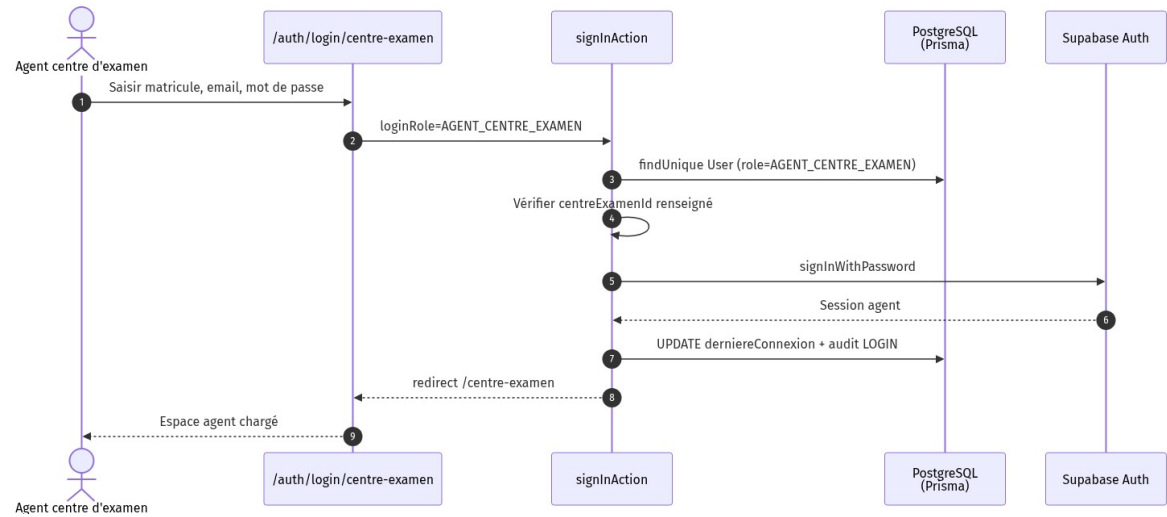
Figure 3.33 — SEQ-AGENT-01 : connexion agent
