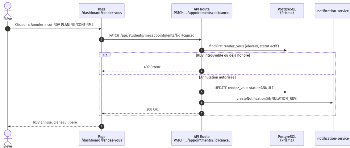
Figure 3.20 — SEQ-ELEVE-10 : annulation RDV
