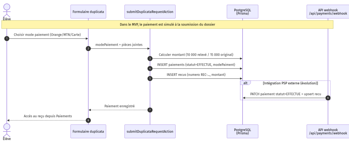
Figure 3.16 — SEQ-ELEVE-07 : paiement duplicata
