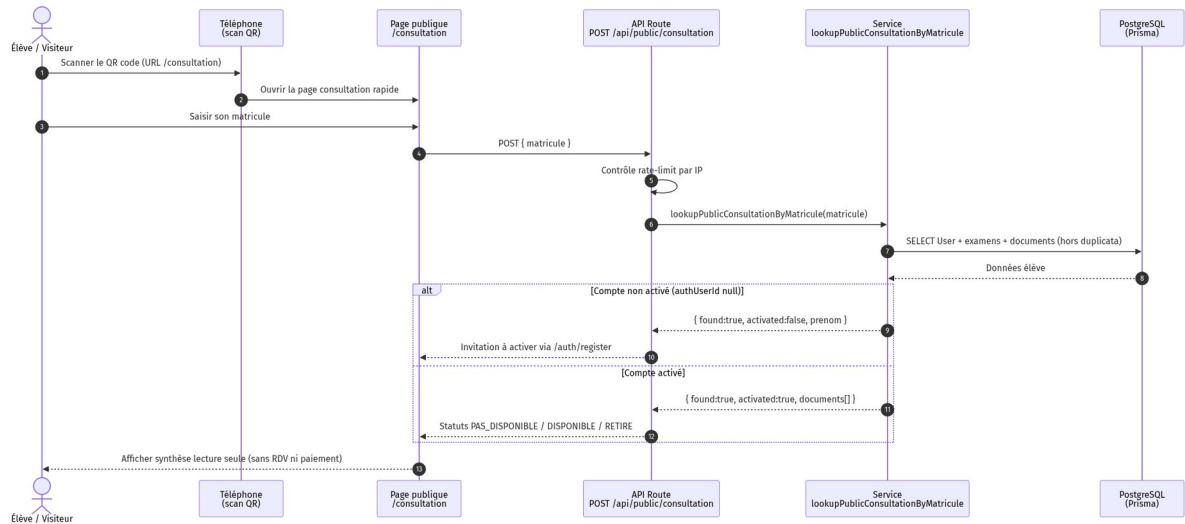
Figure 8.4 — SEQ-ELEVE-02 : consultation publique
