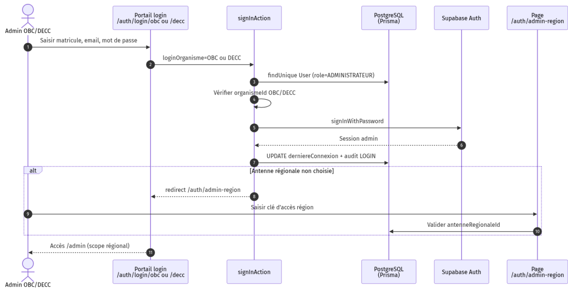
Figure 8.10 — SEQ-ADMIN-01 : authentification administrateur
