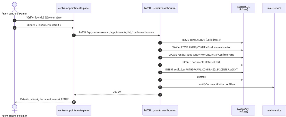
Figure 8.18 — SEQ-AGENT-03 : confirmer retrait
