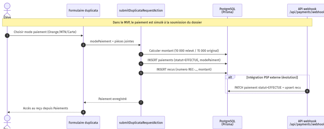
Figure 8.7 — SEQ-ELEVE-07 : paiement duplicata
