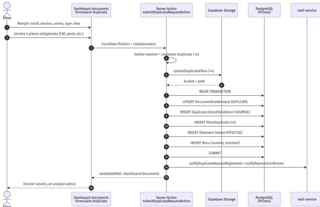
Figure 8.6 — SEQ-ELEVE-06 : formulaire duplicata
