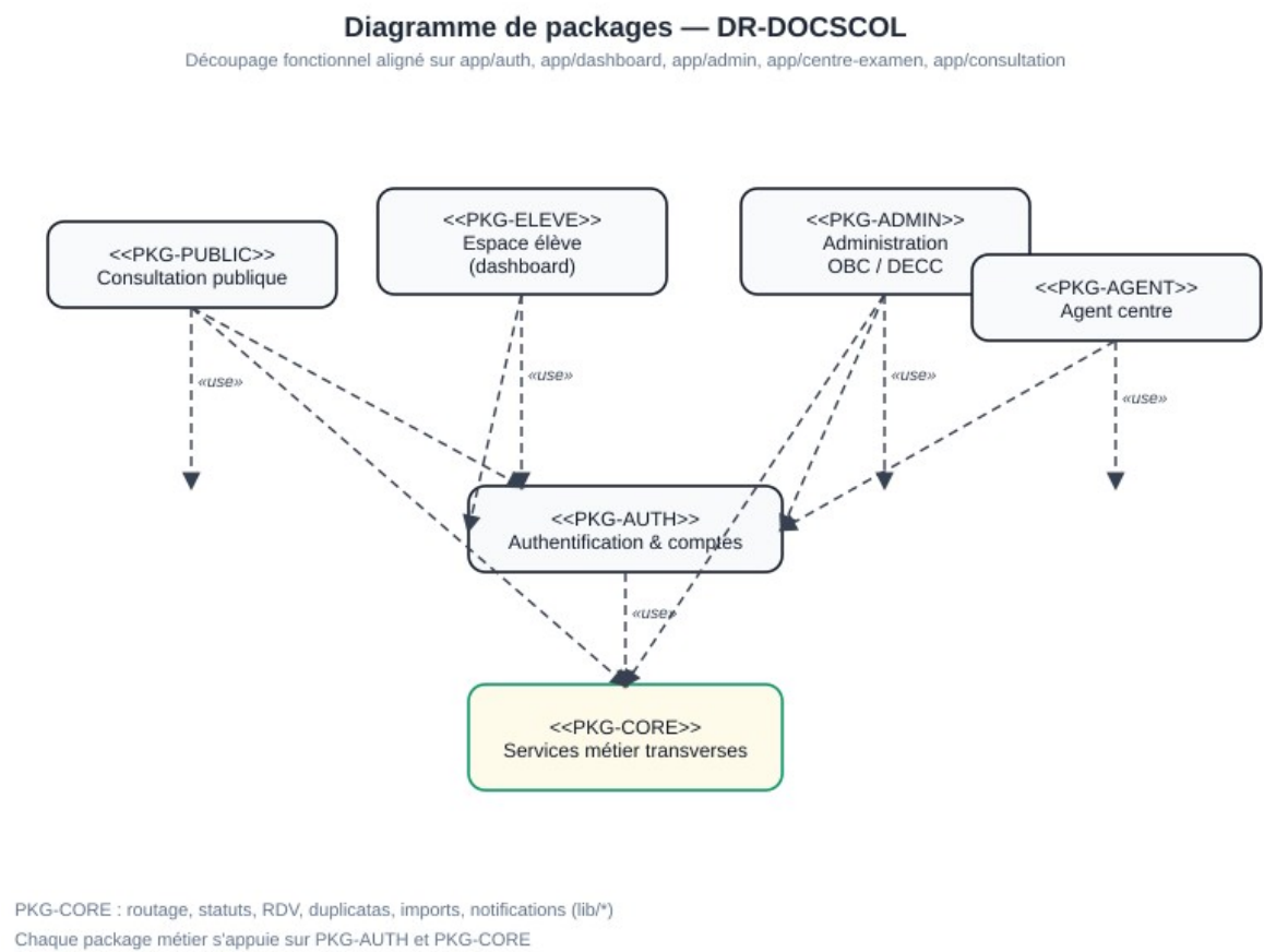
Figure 8.0 — Diagramme de packages DR-DOCSCOL
