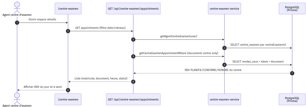
Figure 8.17 — SEQ-AGENT-02 : consulter RDV
