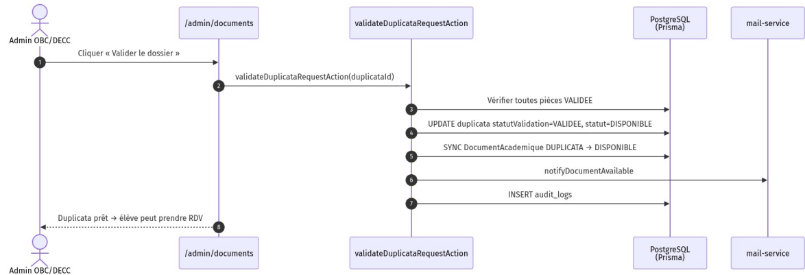
Figure 8.13 — SEQ-ADMIN-08 : valider duplicata
