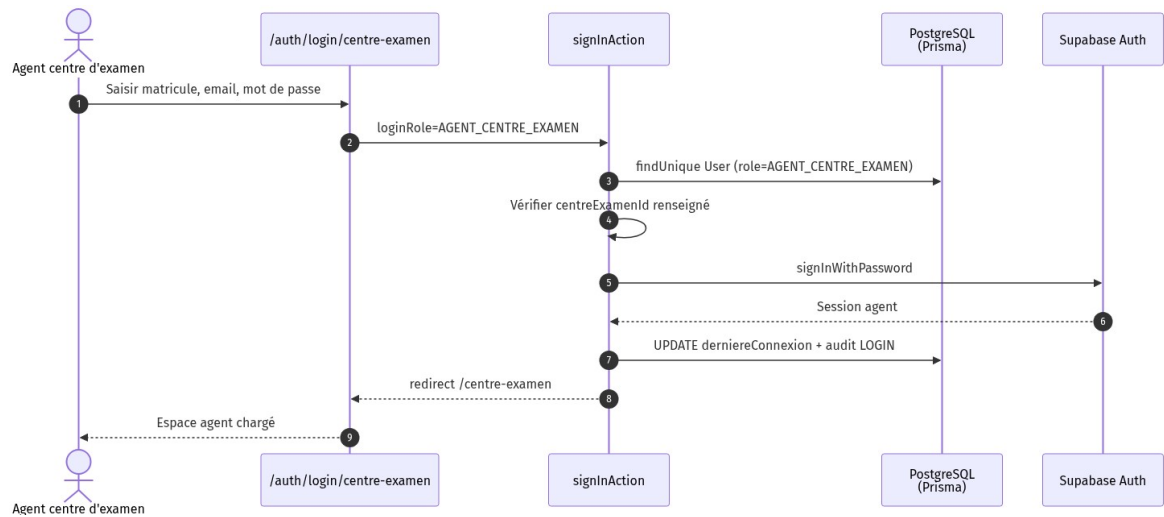
Figure 8.16 — SEQ-AGENT-01 : authentication agent
