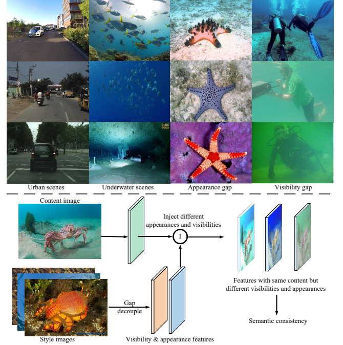
Fig. 1: Visualization of the domain gap in UnderwaterDG (Top) and the core design of our method (Bottom).
