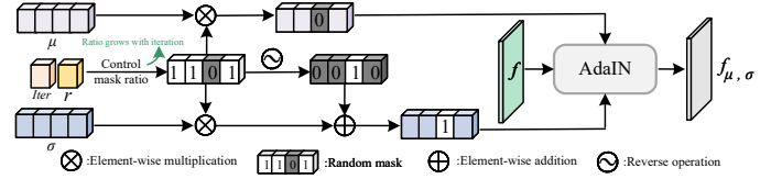
Fig. 5: The overview of CSMP, where curriculum-guided masking is applied to style statistics to simulate incomplete or degraded style conditions, enabling more robust and domain-invariant feature augmentation.
