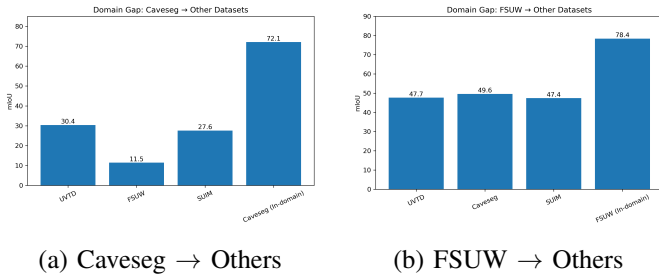
Fig. 8: Quantitative analysis of the domain gap under single-source training using DINOv2.
