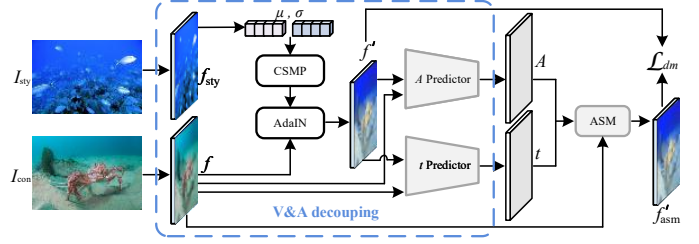
Fig. 3: The illustration of VADM. CSMP and AdaIN generate a stylized feature f' with controlled visibility/appearance changes, while the predictors P_A and P_t extract the corresponding components and reconstruct f'_{asm} through ASM to enforce effective feature decoupling.
