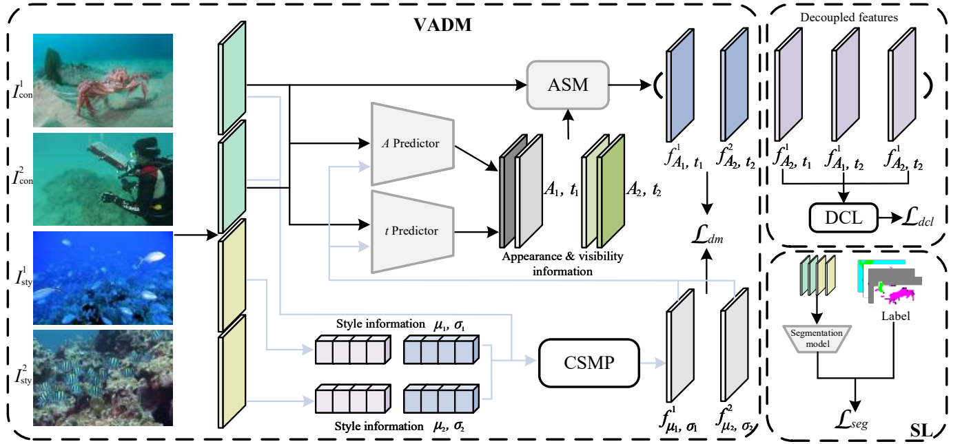
Fig. 2: The overview of our framework. VADM, CSMP, DCL, and SL represent visibility-appearance decoupling modeling, curriculum-guided style-masking perturbation, decoupled consistency loss, and supervised learning, respectively.
