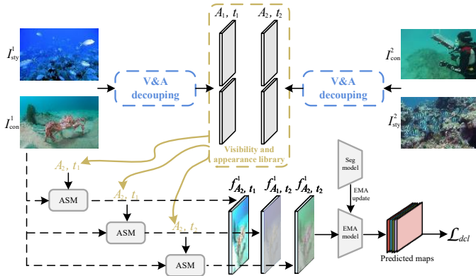
Fig. 4: The illustration of DCL, which applies visibility-only, appearance-only, and combined augmentations with EMA-guided consistency constraints to enforce visibility- and appearance-guided consistency predictions. V&A decoupling operation is parts of VADM, which is shown in Fig. 3. The yellow arrows indicate the different feature variables selected for each augmentation branch. Consistency constraints are enforced via an EMA model derived from the segmentation network.
