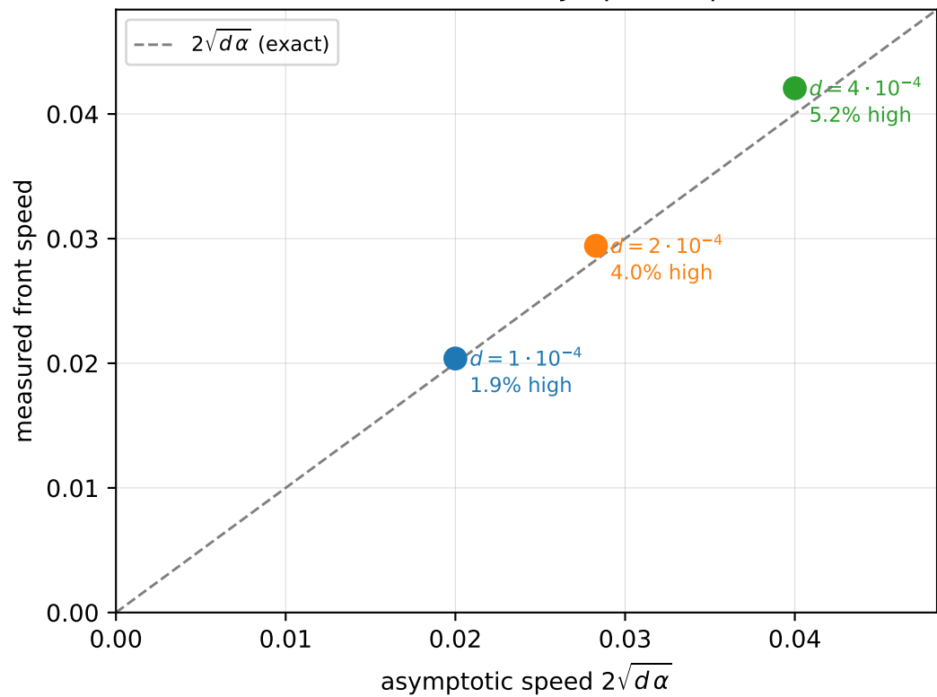
Measured versus asymptotic speed
