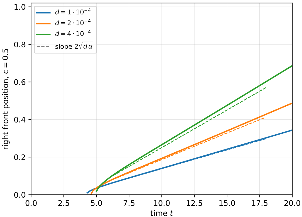
Front propagation at \alpha = 1
