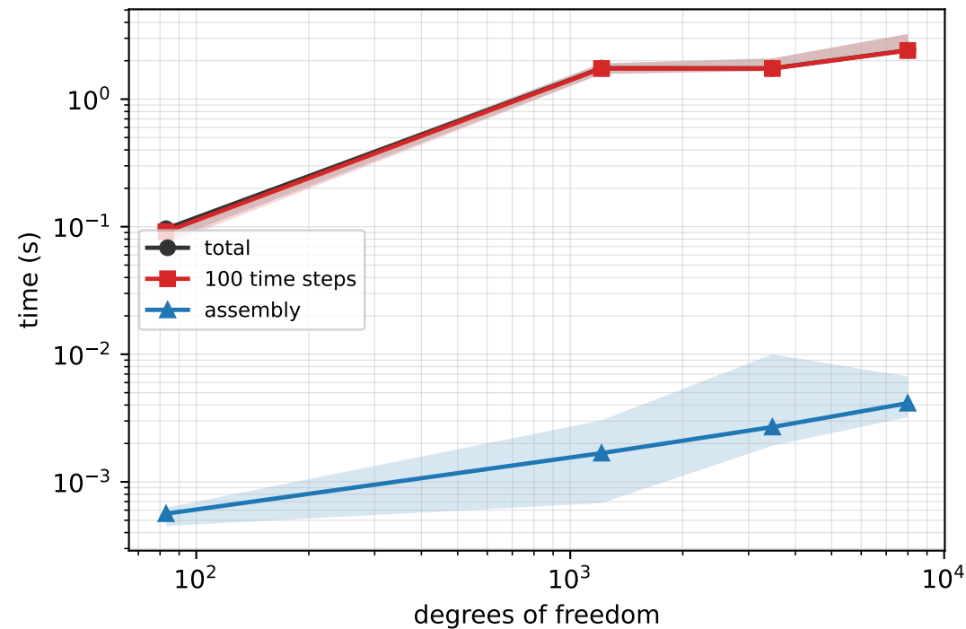
Sequential Corti-83 baseline (median of 5 runs, band = min to max)
