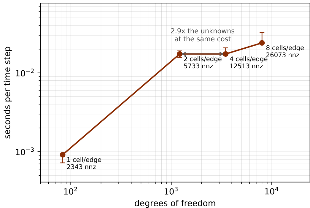
Nonlinear time-step cost is not a function of the unknown count alone
