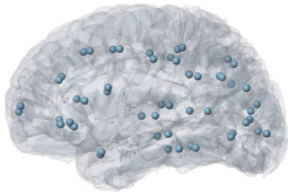
amyloid- \beta seeding
