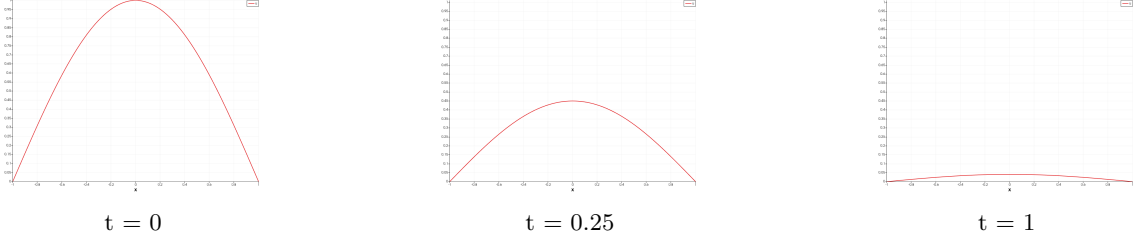
Figure 6: This test considers a radially decaying solution where both the diffusion and reaction term contribute to the temporal dynamics of the solution. The Backward Euler scheme is used and a mesh size h = 0.01 .
