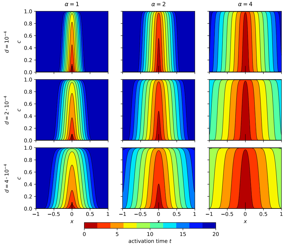
Figure 18: Activation-time maps for the one dimensional Fisher–Kolmogorov problem. The reaction coefficient increases from left to right, while the diffusion coefficient increases from top to bottom. For each pair (x, c) , the color represents the first time at which the numerical concentration at x reaches a particular level c ; black curves denote equal activation times. All panels use the same time scale t \in [0, 20] .
