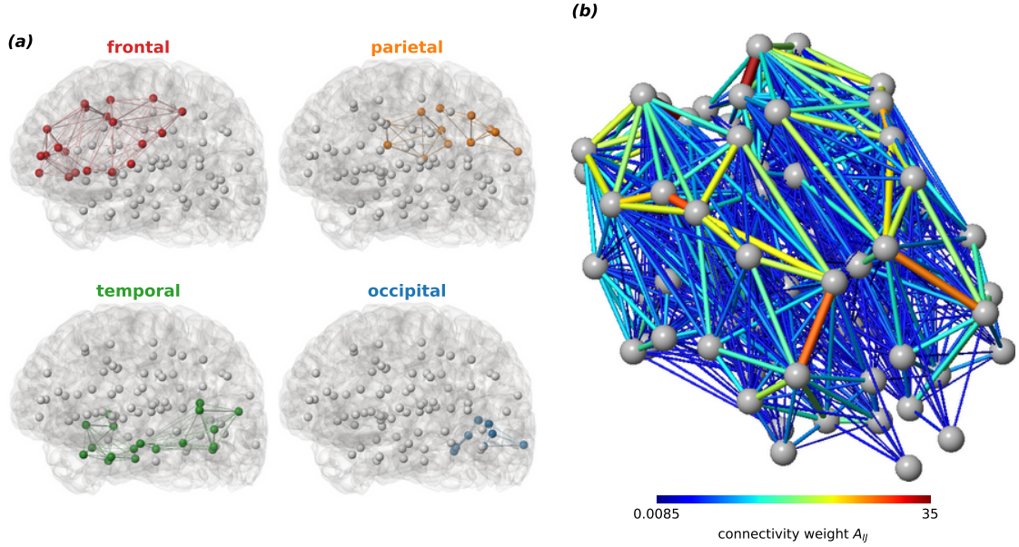
Figure 21: (a) The four cortical lobes: the regions of a lobe are coloured and the connections internal to it are drawn; white vertices belong to the remaining regions of a finer classification. (b) The resulting graph in the oblique view without the pial surface, connections coloured by connectivity weight. This is the abstract object the finite element method computes on; since an aggregated connection has no unique physical length, we choose for every edge a unit metric length: the anatomical information enters through its weight, the vertex coordinates being used for visualization only.
