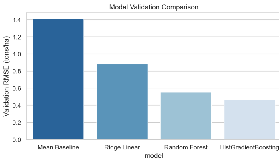
Figure 10 (fig10_model_comparison.png): Validation RMSE by model. Takeaway: error falls at each step from the mean baseline to Ridge, Random Forest and HistGradientBoosting, which is lowest.
