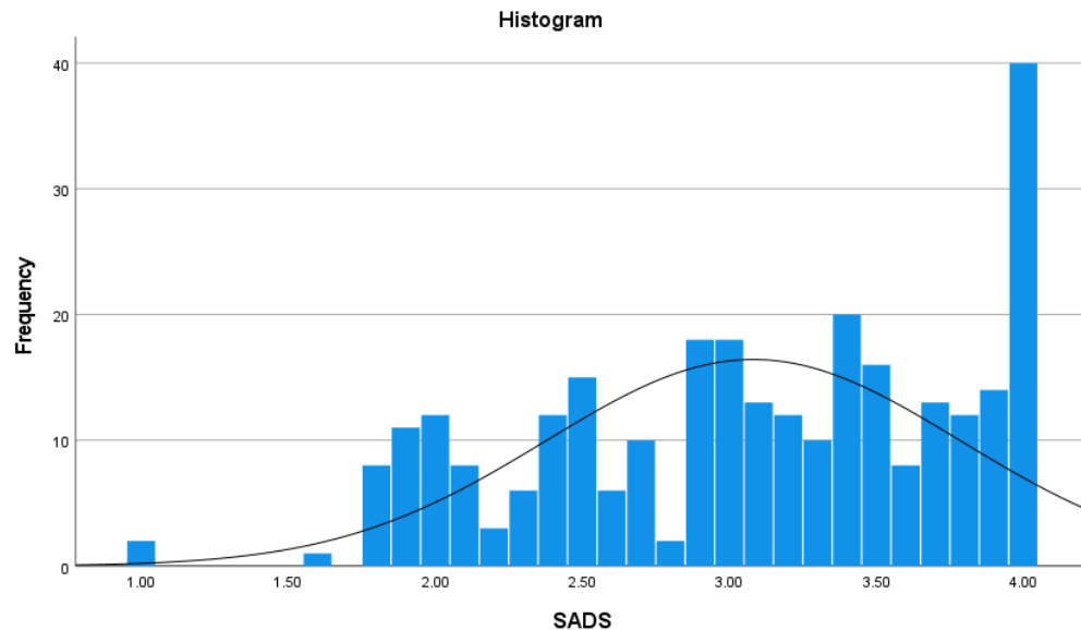
Fig. 4: The normal distribution of the SADS
