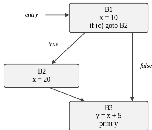
Figure 2. Basic blocks and control-flow graph for an if/else statement.
