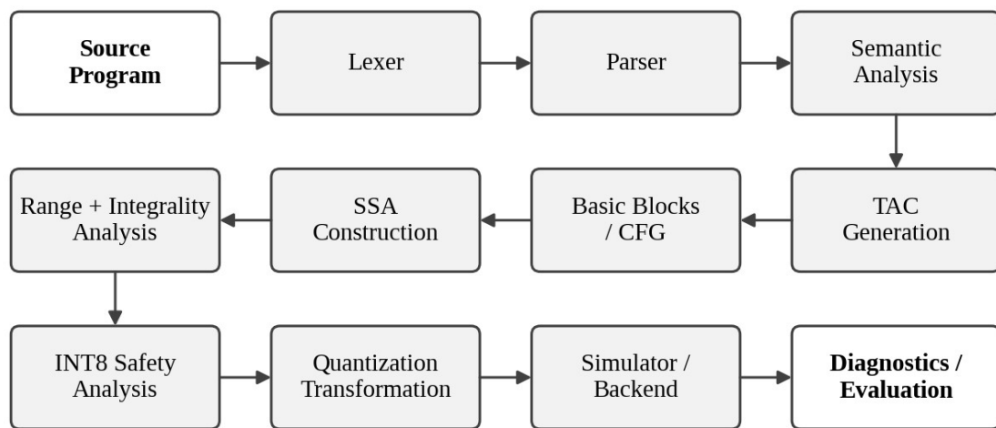
Figure 1. Overall compiler pipeline, from source program to diagnostics.
