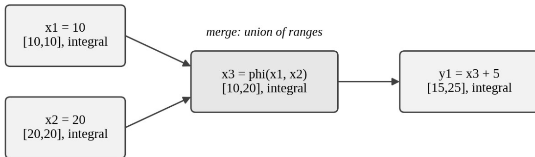
Figure 4. Range propagation through a phi node and a subsequent addition.
