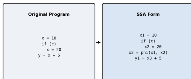
Figure 3. Original program and its static single assignment form.
