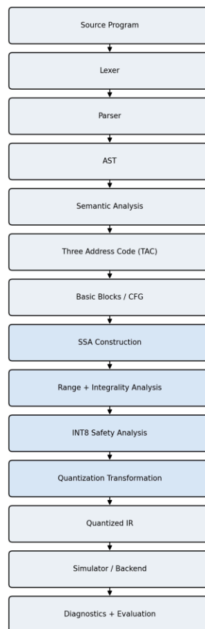
Figure 1. Overall compiler pipeline, from source program to diagnostics.
