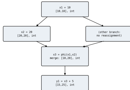
Figure 4. Range propagation through a phi node and a subsequent addition.
