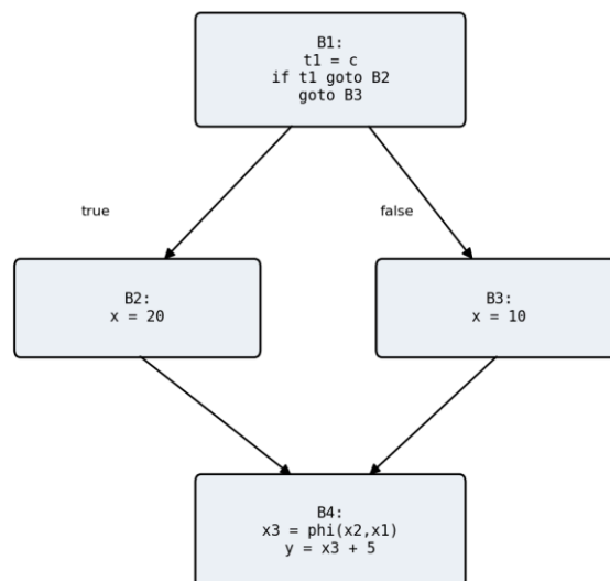
Figure 2. Basic blocks and control-flow graph for an if/else statement.
