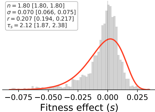
REL606
