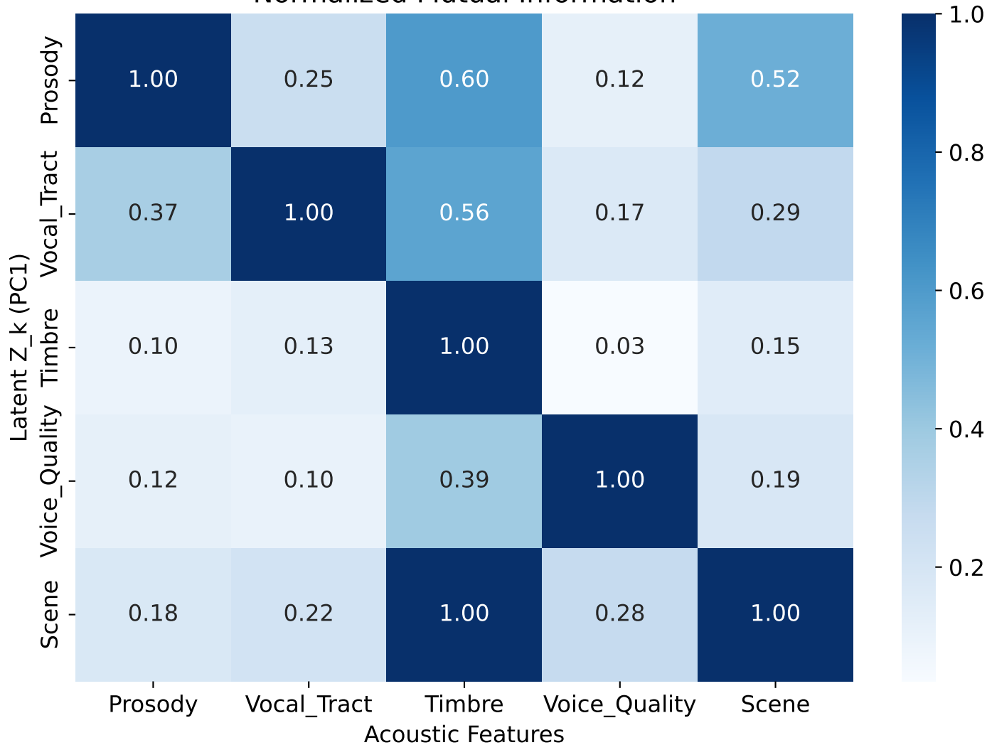
Normalized Mutual Information
