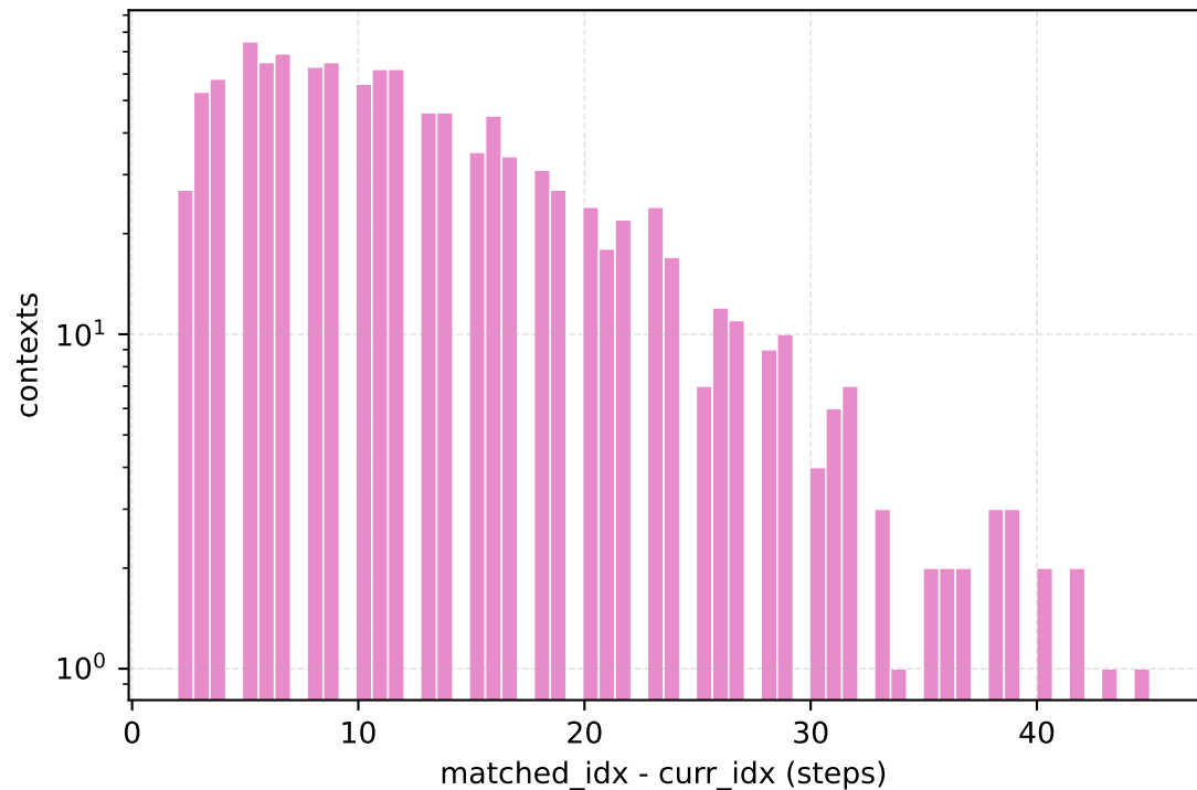
Fuzzy context step distance (matched) match=1.000
