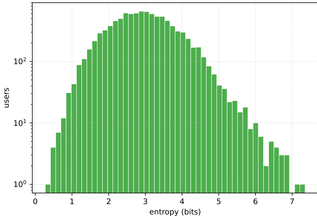
User visit entropy H(\text{grid} \mid \text{user})
