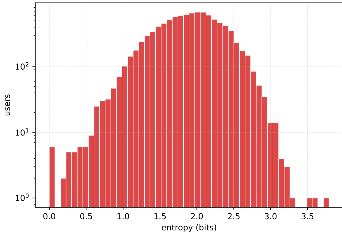
User conditional transition entropy H(\text{next} \mid \text{curr}, \text{user})
