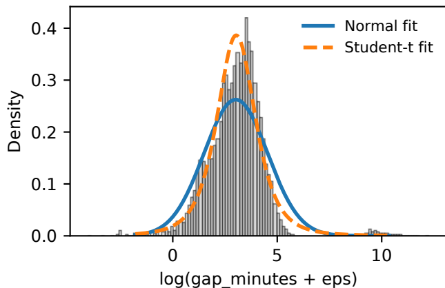
(c) MoreUser: log gaps + fits
