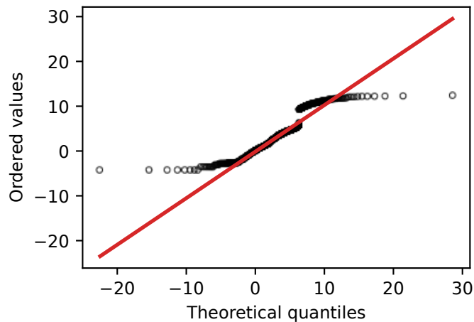
(b) GeoLife: QQ vs Student-t
