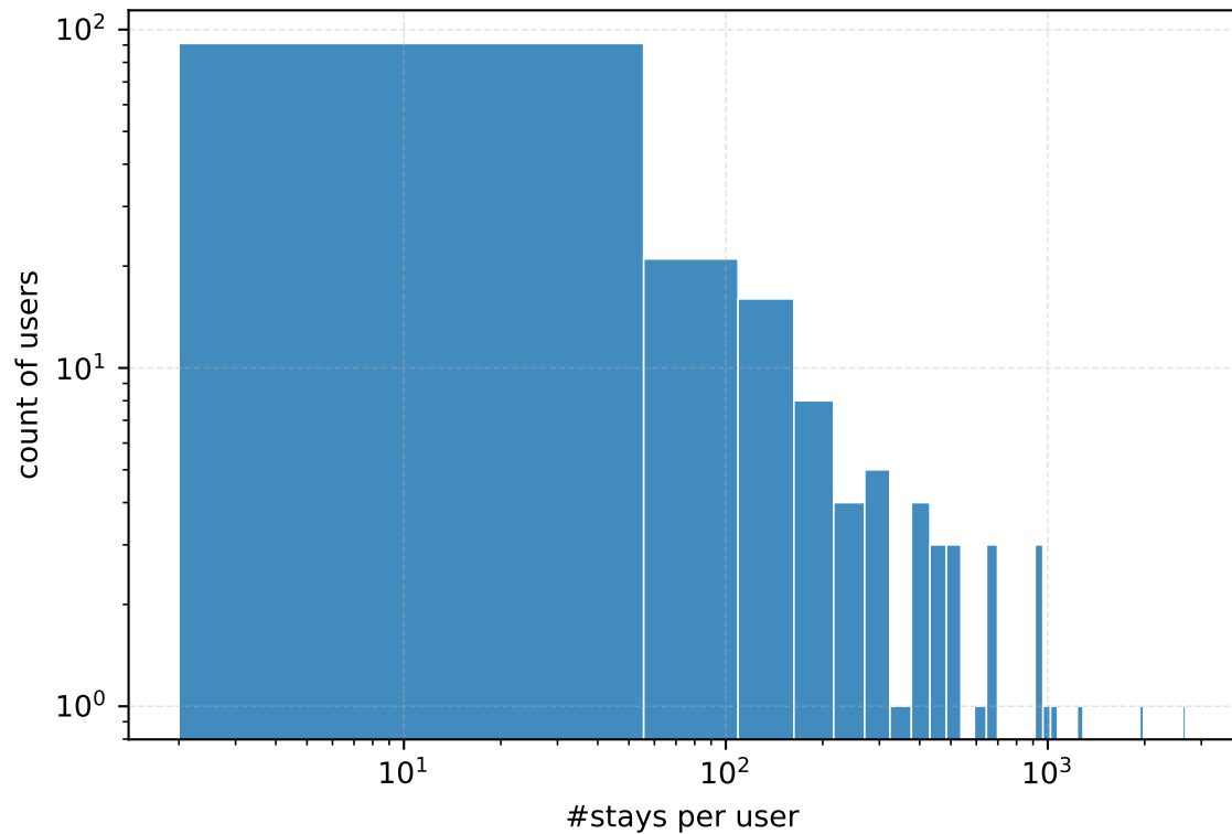
Stays per user (log-log) | users=168, stays=27914
