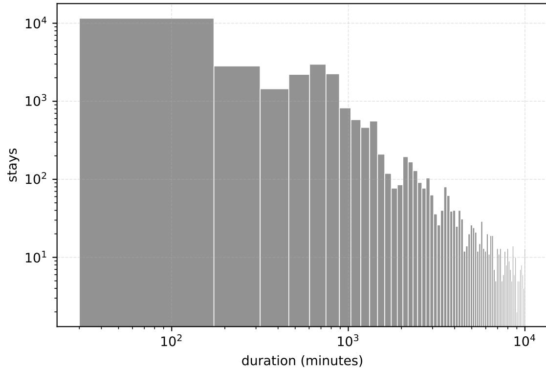
Stay duration distribution (log-log)
