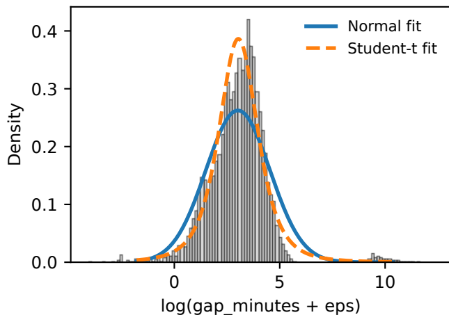
(a) GeoLife: log gaps + fits
