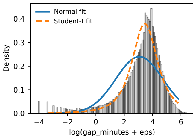
(c) MoreUser: log gaps + fits
