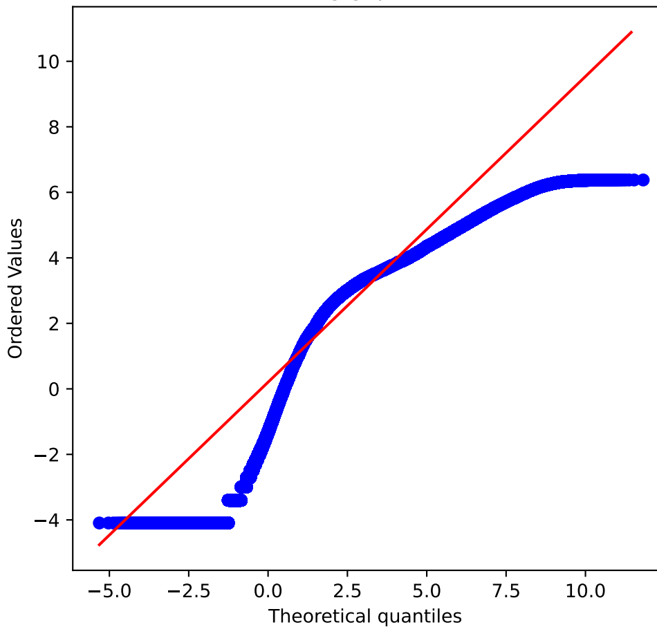
QQ-Plot: log gaps vs Normal
