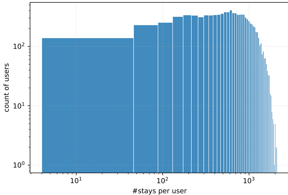
Stays per user (log-log) | users=9907, stays=6818428
