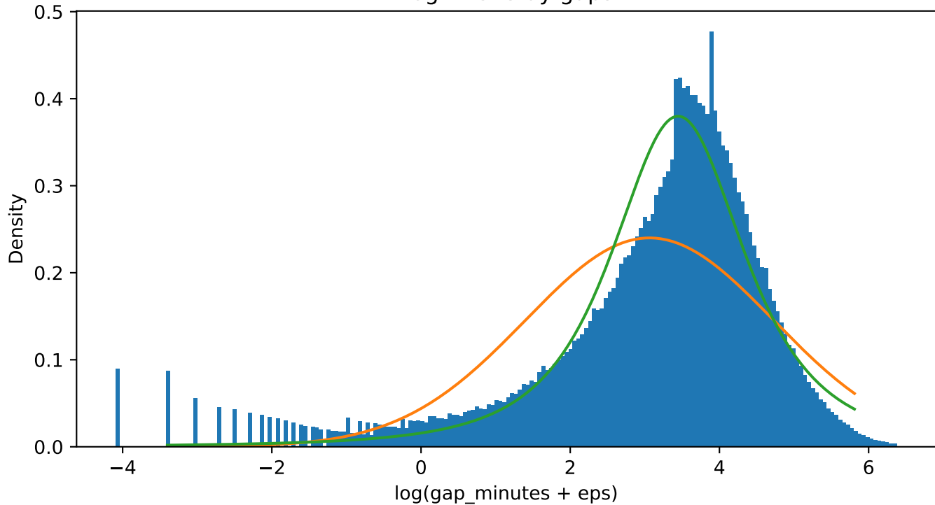
Log inter-stay gaps
