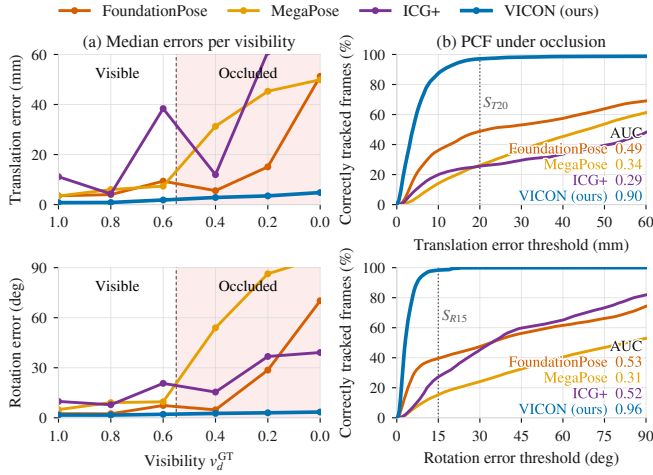
Fig. 5. Object-pose errors over the 40 motion-capture sessions (top: translation; bottom: symmetry-aware rotation). (a) Median error of each tracker binned by the visibility v_d^{GT} ; shading marks the occluded range. (b) PCF on the 24,285 occluded frames as a function of the error threshold; dotted lines mark the 20 mm and 15° thresholds used for S_{T20} and S_{R15} , and the numbers give the AUC. Medians are used in (a) because diverging baseline errors would dominate a mean.
