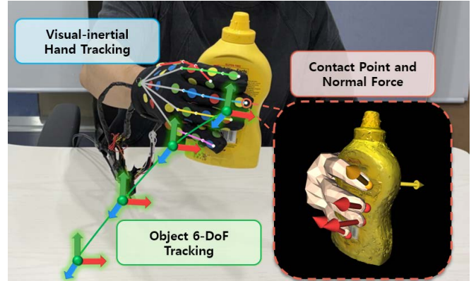
Fig. 1. VICON records hand motion, object pose, contact points, and forces using a visual-inertial glove [1] with integrated FSRs and a single RGB-D camera. The glove tracks the hand skeleton, and our offline refinement maintains robust and accurate object 6-DoF tracking even under severe occlusion. Inset: object-frame contact points, with arrows colored by calibrated normal force magnitude.
