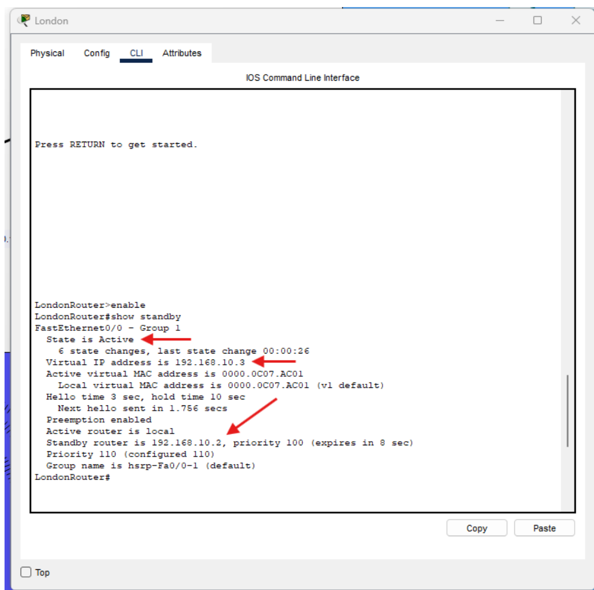
Figure 12: London main router will be the active router.
