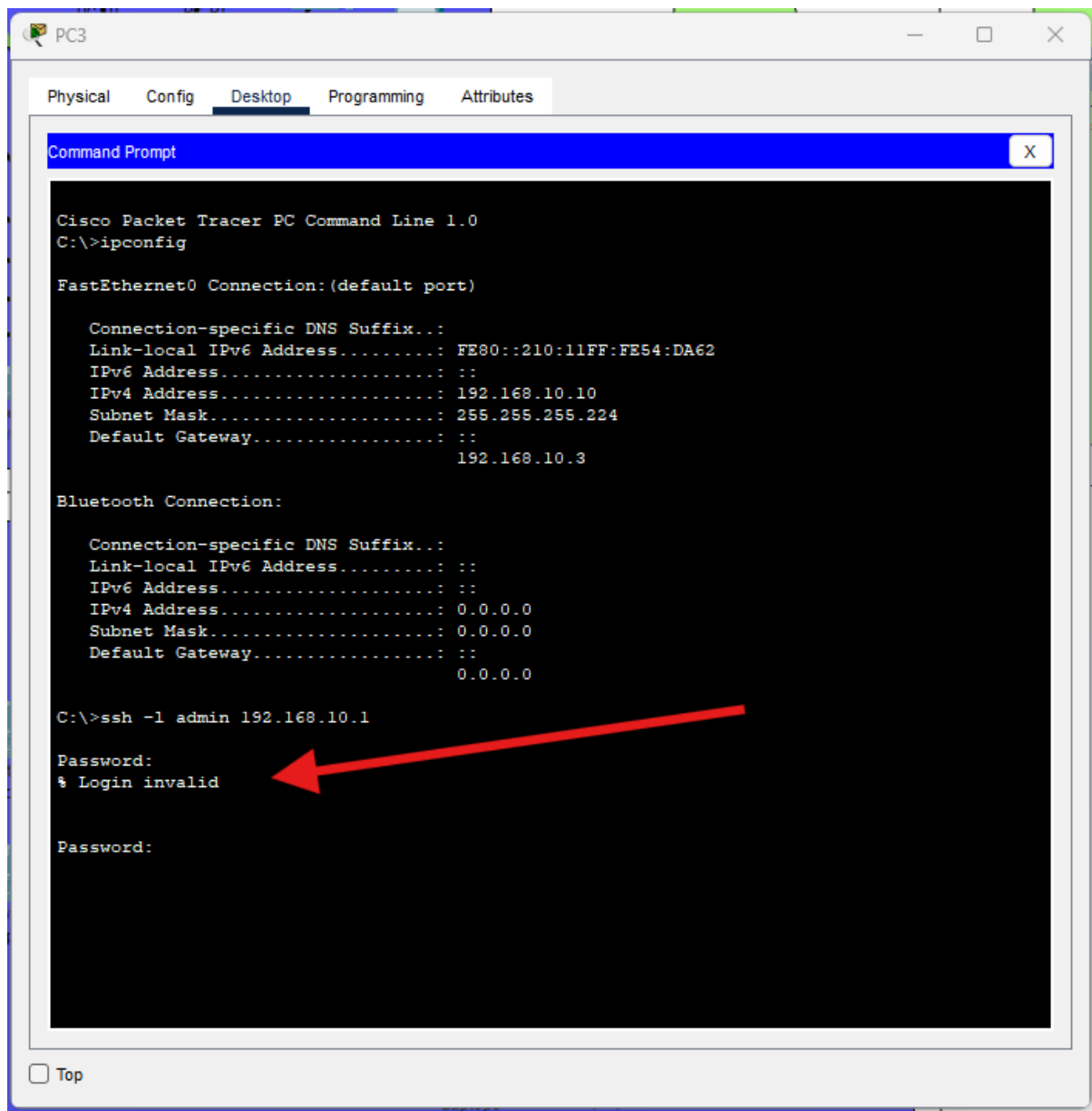
Figure 11: test SSH and input wrong password.
