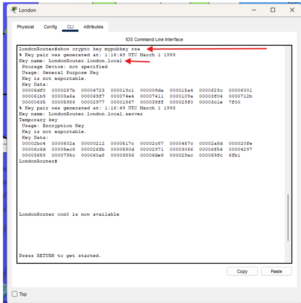
Figure 9: check if the SSH configuration was done correctly with command show crypto key mypubkey rsa .
