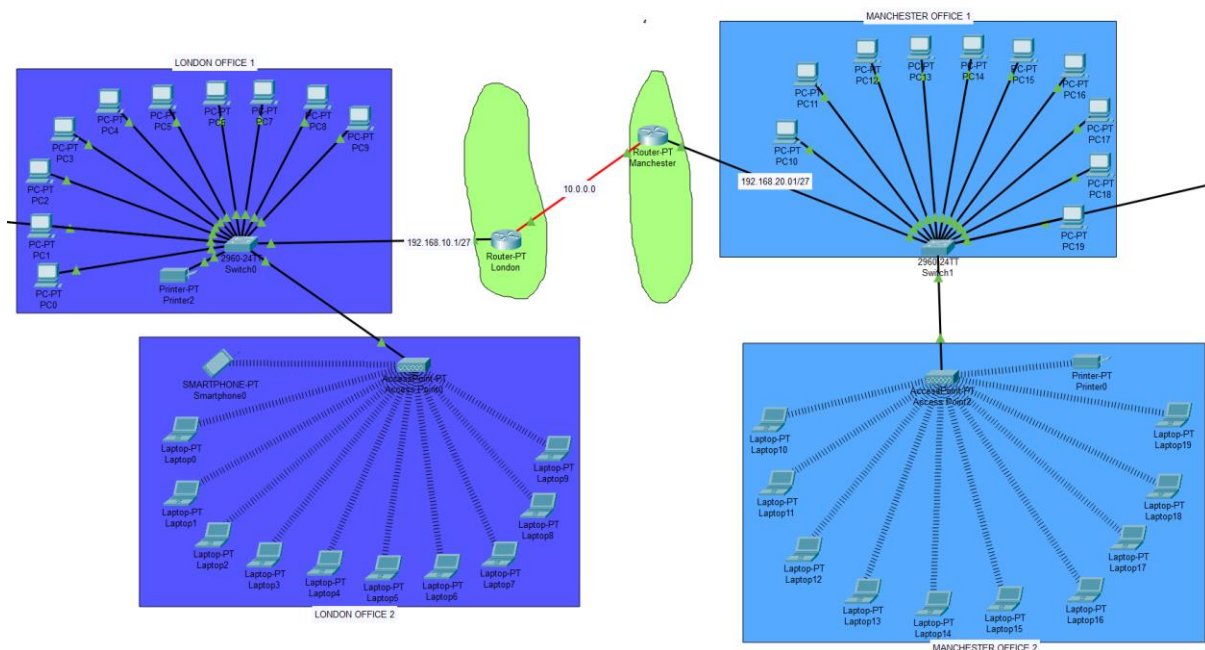
Figure 3: entire network design.
