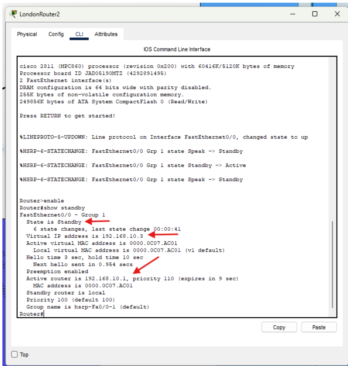
Figure 13: London router 2 will be the router on standby.
