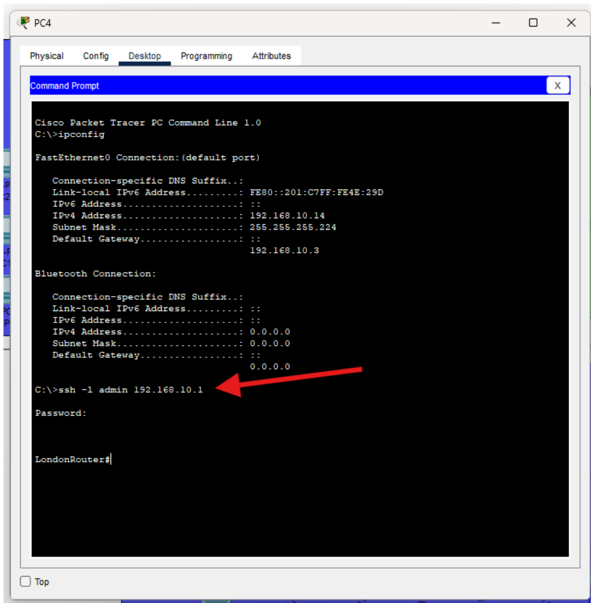
Figure 10: test the SSH configuration and input the correct password
