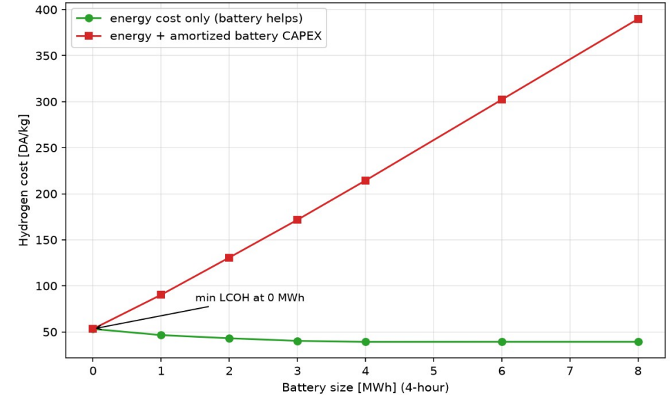
Battery sizing — Ghardaïa clear summer, 280 kg/day CAPEX 250 $/kWh, CRF 0.133 → 12.3 DA/kWh/day
