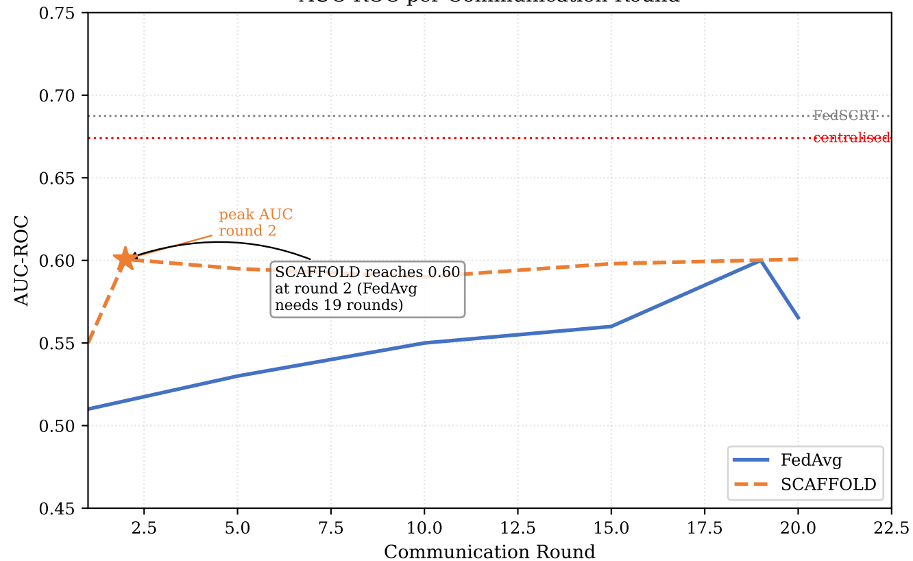
AUC-ROC per Communication Round
