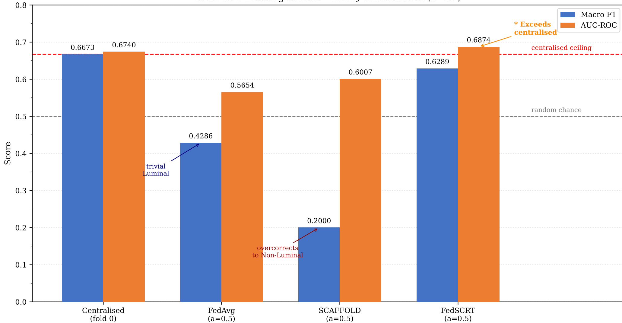
Federated Learning Results -- Binary Classification ( \alpha=0.5 )
