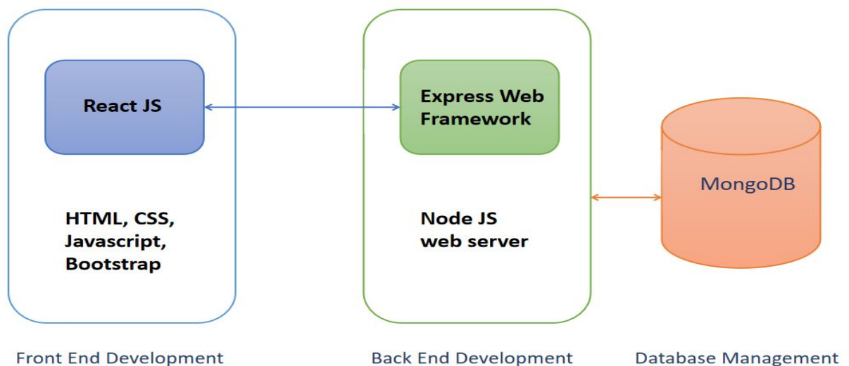
Figure 4.2: System Architecture for YouDescribe Website Application
