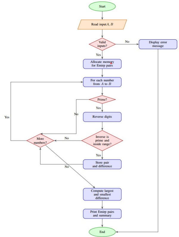
Fig. 1: Flowchart of the implemented Emirp number detection algorithm.
