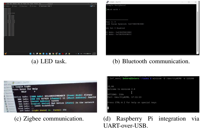
Fig. 9: Experimental results obtained from the RTOS implementation. [2]
