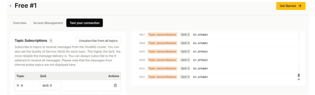
Fig. 6: MQTT broker receiving published sensor measurements. [2]
