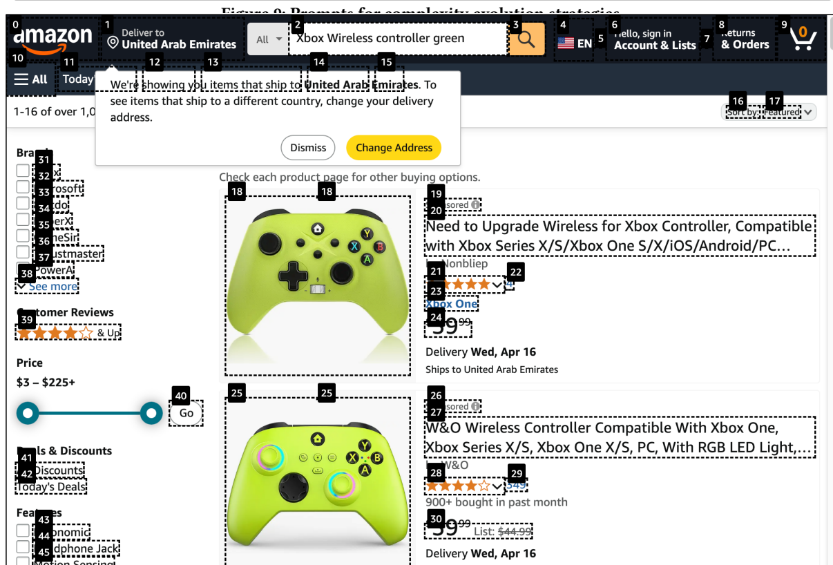
Figure 10: Limited grounding ability of web agents.
