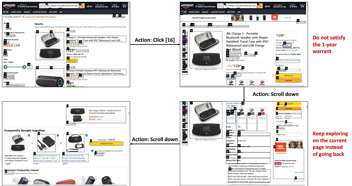
Figure 11: Illustration of web agent's failure to reassess and replan.
