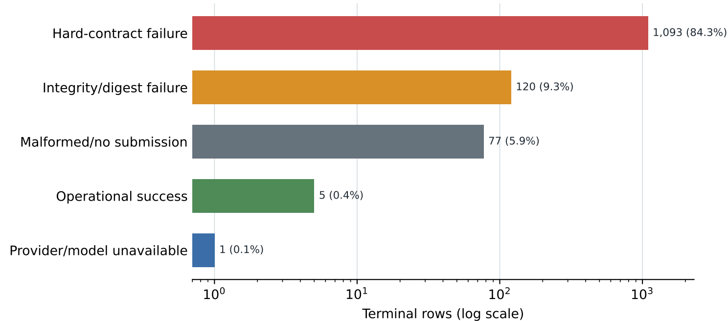
(a) Exact terminal outcomes
