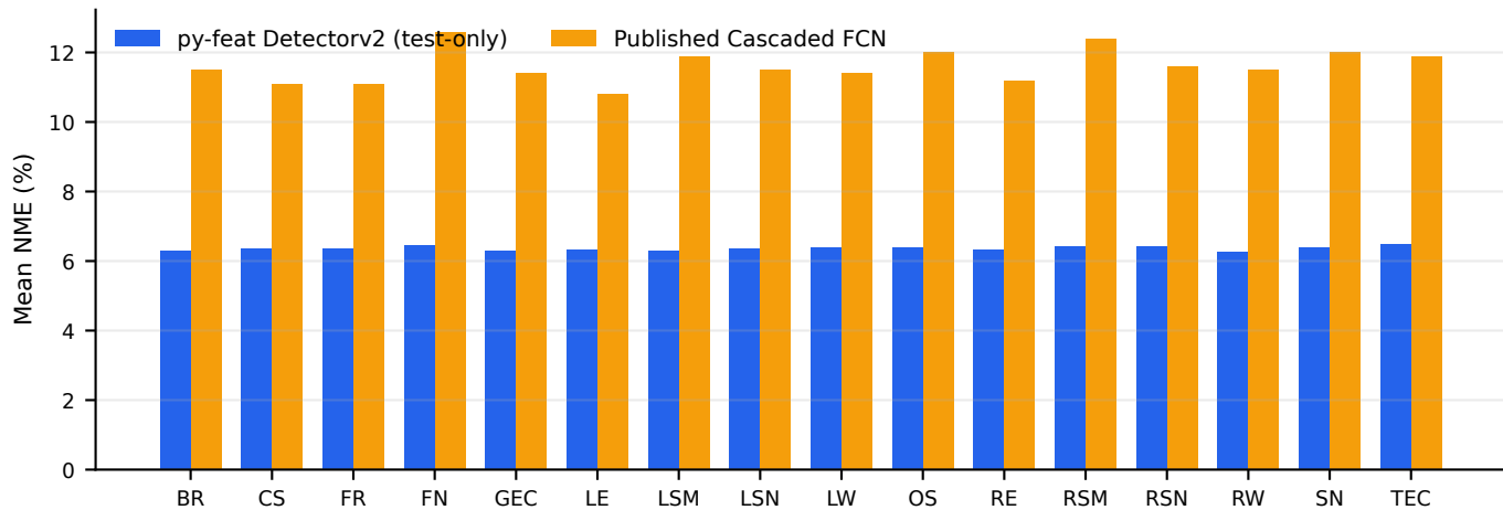
(b) Descriptive comparison of movement means
