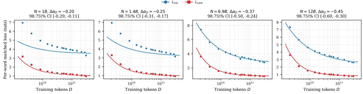
Figure 2: D-axis per-class scaling law at fixed N \in \{1\text{B}, 1.4\text{B}, 6.9\text{B}, 12\text{B}\} . Markers: per-word matched mid-decade loss across 13–14 dense intermediate Pythia checkpoints. Curves: best-fit L = A \cdot D^{-\alpha_D} + E per class. Title under each panel reports the per- N \Delta\alpha_D point estimate with Bonferroni-corrected 98.75% CI. All four CIs exclude zero; magnitude grows from -0.20 at N=1\text{B} to -0.45 at N=12\text{B} .
