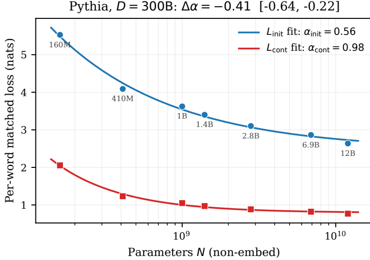
Figure 1: N-axis per-class scaling law at D=300B on the 7 non-anomalous Pythia sizes (160M–12B). Markers: per-word matched mid-decile loss. Curves: best-fit L = A \cdot N^{-\alpha} + E per class. \Delta\alpha = \alpha_{init} - \alpha_{cont} = -0.41 , 95% bootstrap CI [-0.64, -0.22] ; 0 of 2000 bootstrap draws had \Delta\alpha \geq 0 (i.e. P(\Delta\alpha \geq 0) < 5 \times 10^{-4} ).
